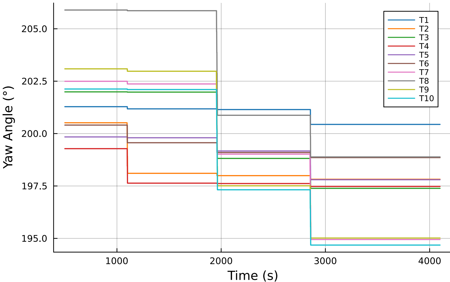
Turbine Yaw Angles vs Time
