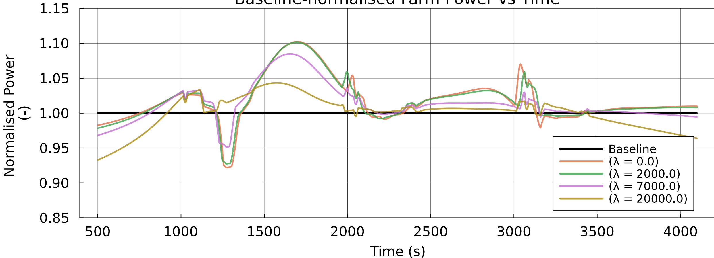
Baseline-normalised Farm Power vs Time
