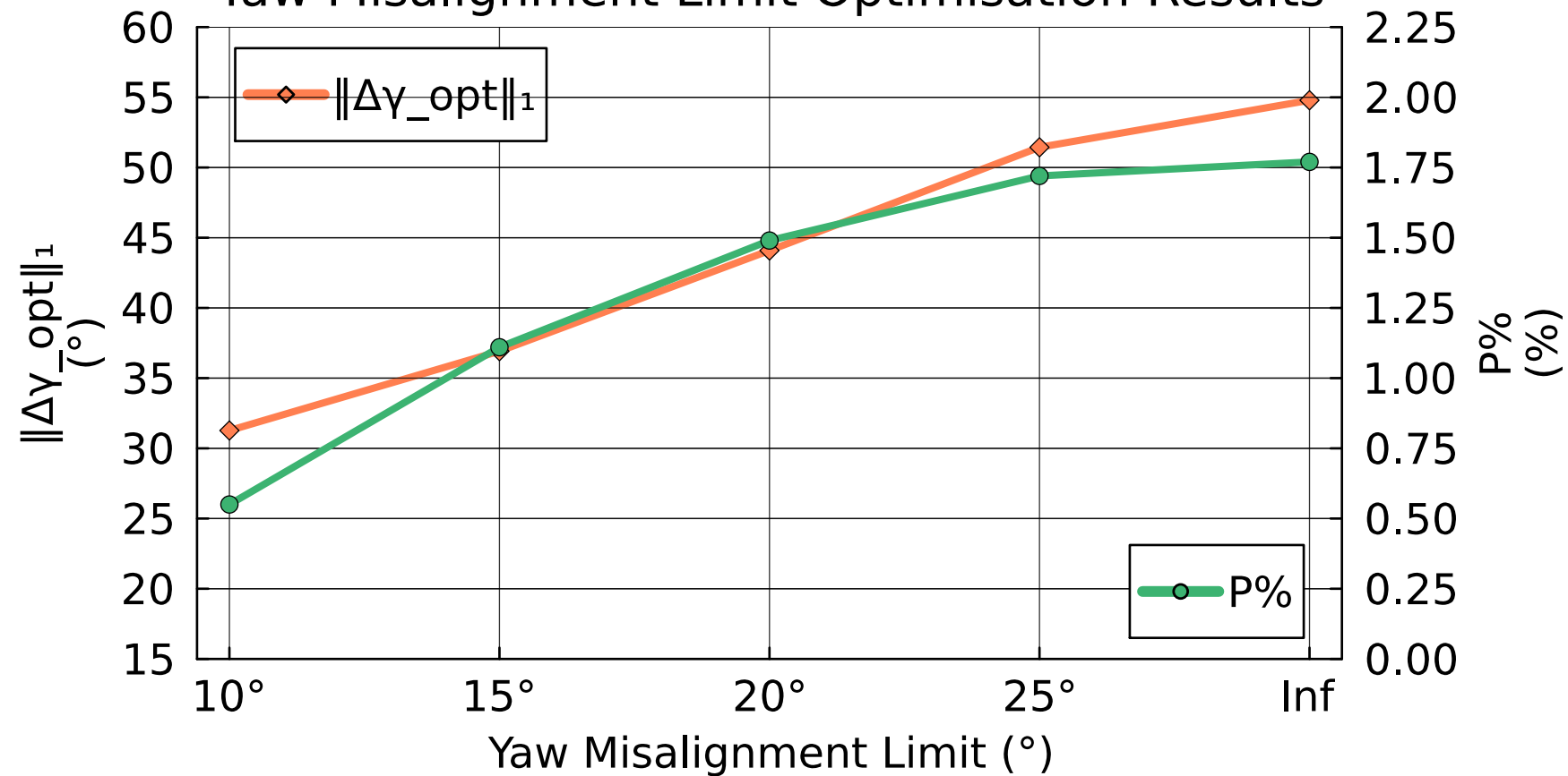
Yaw Misalignment Limit Optimisation Results
