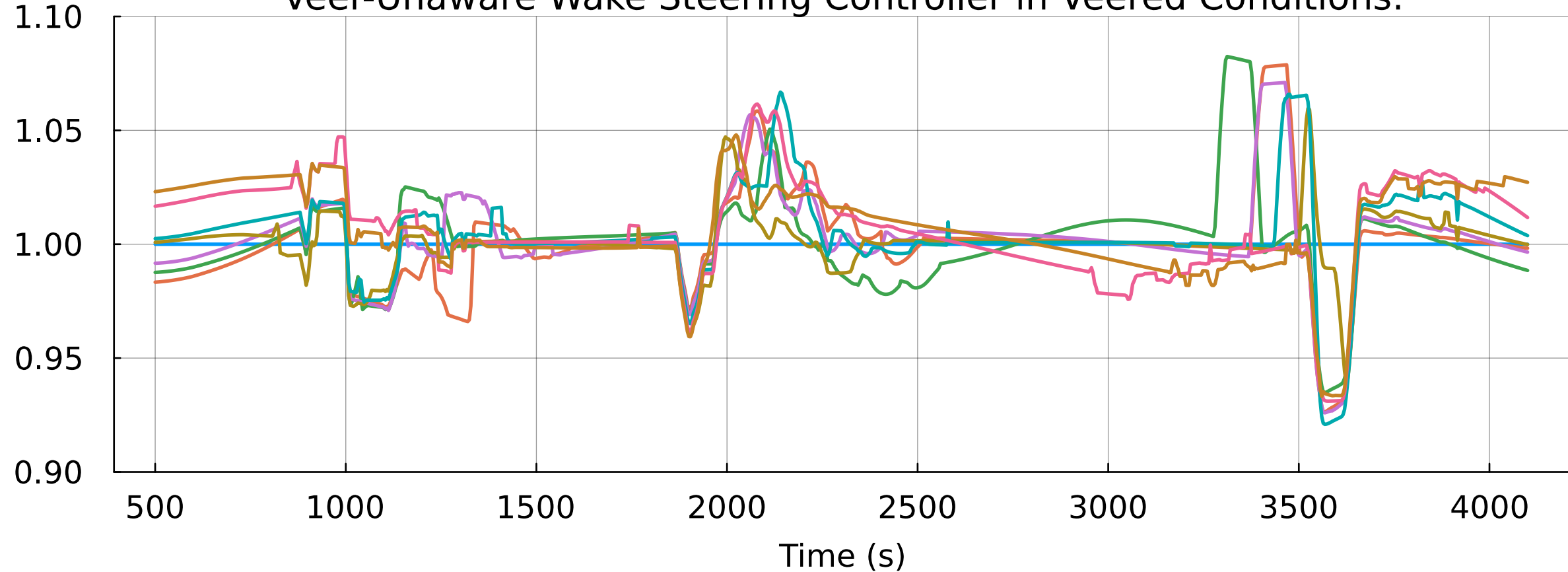
Veer-Unaware Wake Steering Controller in Veered Conditions:
