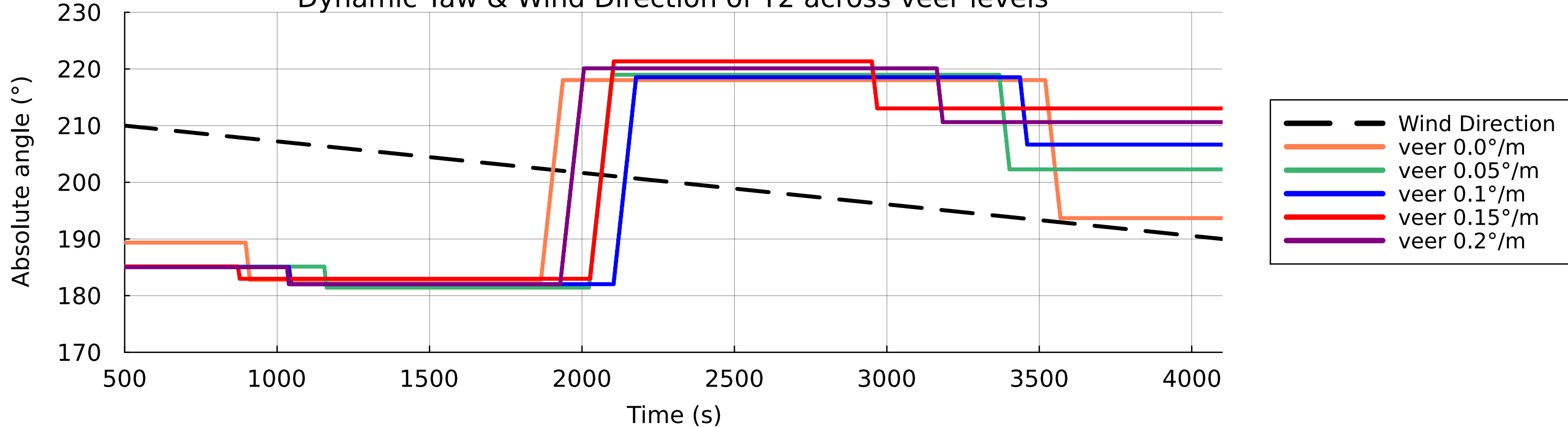
Dynamic Yaw & Wind Direction of T2 across veer levels
