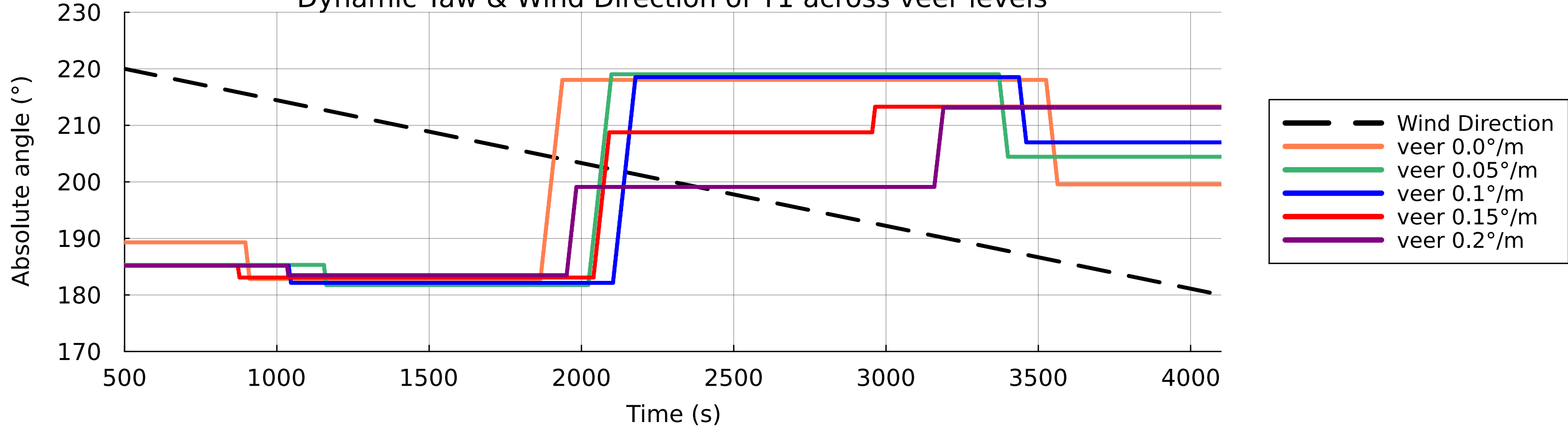
Dynamic Yaw & Wind Direction of T1 across veer levels
