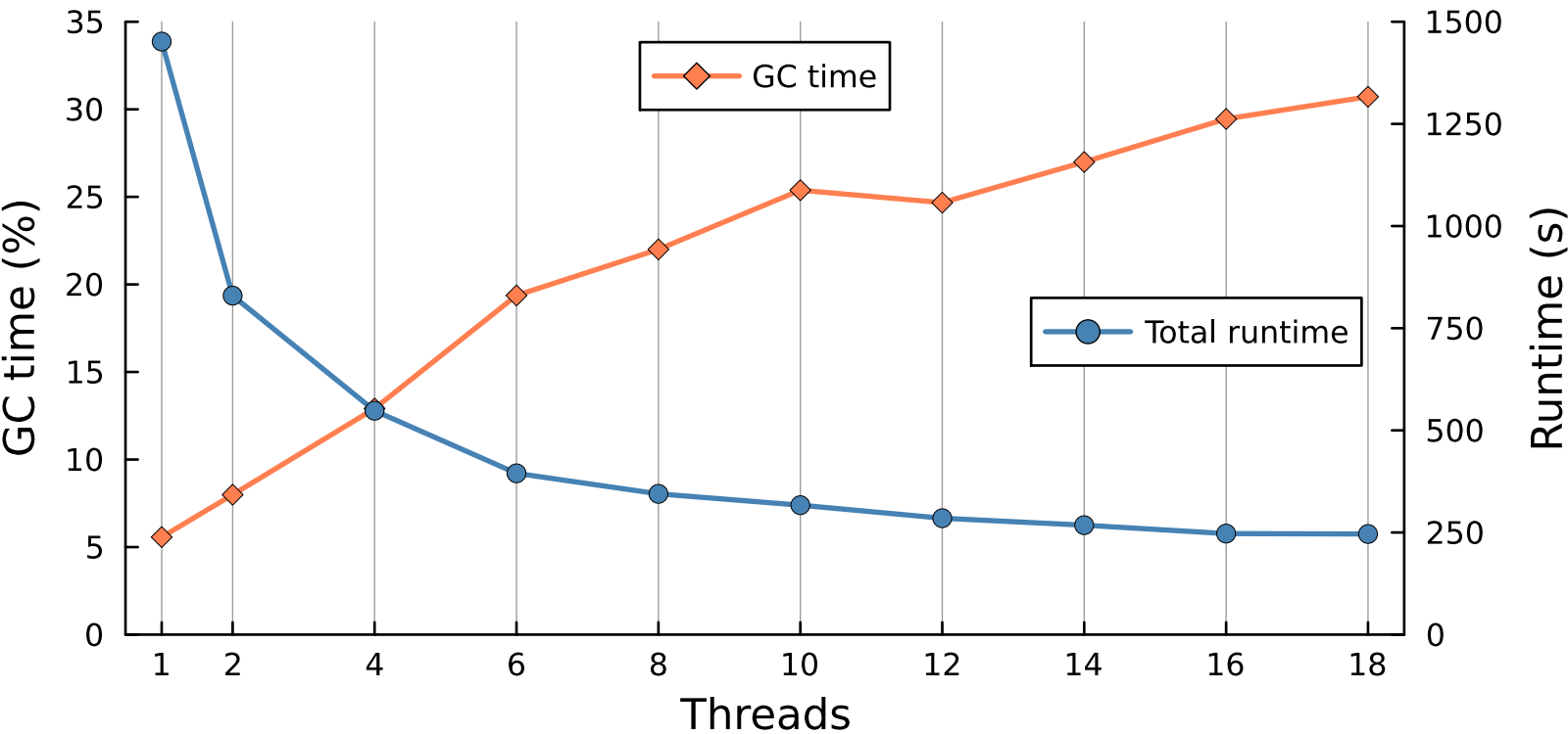
Runtime & GC Time % vs. Thread Count
