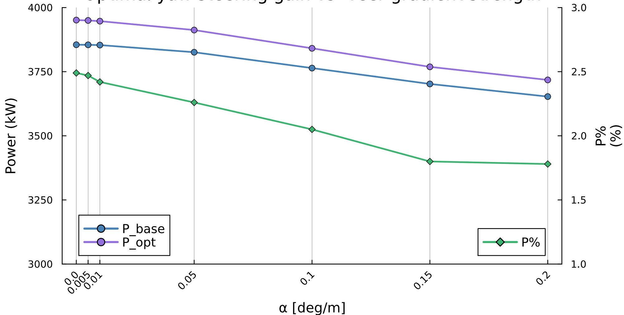
Optimal yaw steering gain vs. Veer gradient strength
