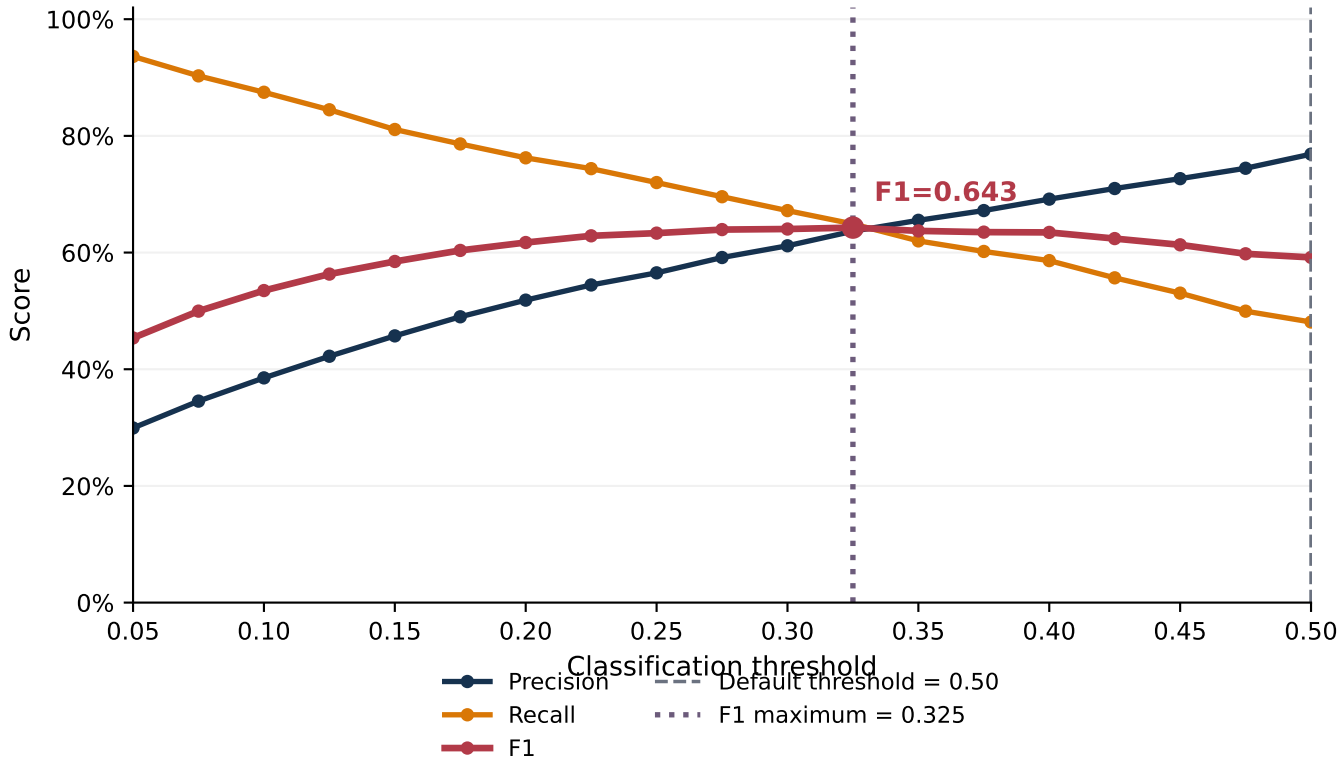
Brazil gradient boosting: threshold tradeoff
