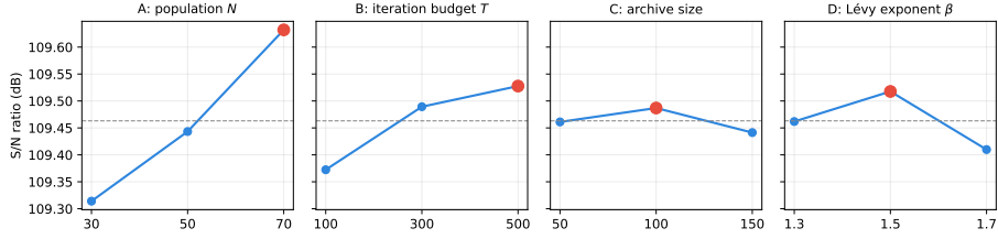
Fig. 1. Main-effects plot of the S/N ratio. The dashed line is the grand mean (109.46 dB) and the red marker the best level per factor; population and iteration budget show clear trends (population the steeper), while archive size and \beta are essentially flat.
