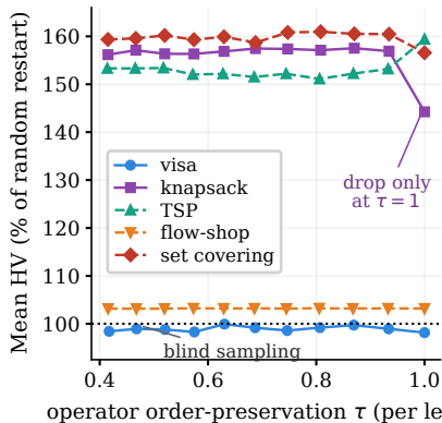
(a) hypervolume
