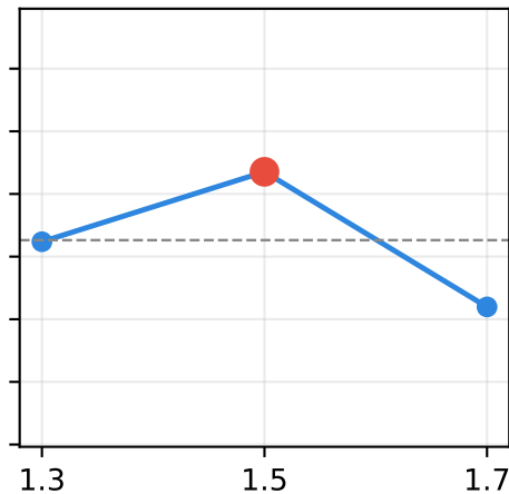
D: L\'evy exponent \beta
