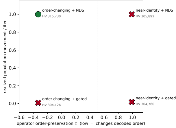
Fig. 8. Mechanism of the two conditions across the 2 \times 2 cells: operator order-preservation \tau (x) versus realized population movement per iteration (y), with each cell’s mean HV annotated. Only the order-changing, diversity-preserving cell occupies the favorable low- \tau , high-movement corner and beats blind sampling.
