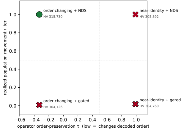
Fig. 9. Mechanism of the two conditions across the 2 \times 2 cells: operator order-preservation \tau (x) versus realized population movement per iteration (y), with each cell’s mean HV annotated. Only the order-changing, diversity-preserving cell occupies the favorable low- \tau , high-movement corner and beats blind sampling.
