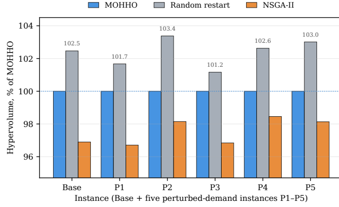
Fig. 10. Generalization over six instances (base plus five \pm 20\% perturbed-demand instances, P1–P5), each method’s mean hypervolume shown as a percentage of MOHHO’s on that instance. The ranking random restart \geq MOHHO > NSGA-II is preserved throughout (101–103 % vs. 96–99 % of MOHHO); on every instance the combined front also dominates the FIFO baseline (not shown).
