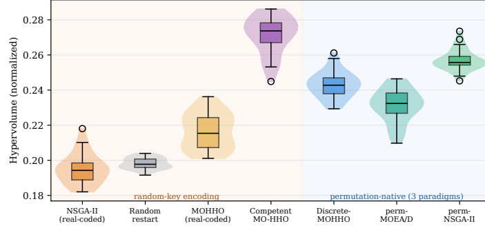
Fig. 11. The seven-method ladder on the multidimensional knapsack (MOMKP), one of the four structures of Table 9. The naive random-key methods (NSGA-II and random restart) sit below the permutation-native methods, while the competent random-key swarm is the single best method here (mean rank 1.13 of seven)—so the divide is non-degenerate search, not the encoding. The split reverses only on the sequencing landscapes (TSP, flow-shop), where the real-coded GA becomes competitive (Table 9).
