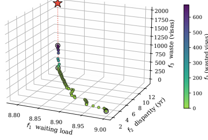
Fig. 2. The 104-solution combined Pareto front over the three objectives, colored by the waste f_3 . The FIFO baseline (red star, the isolated marker above the surface) floats above the front—the dotted drop-line marks its distance to the front’s waste level—and is dominated; circles mark the extreme solutions.
