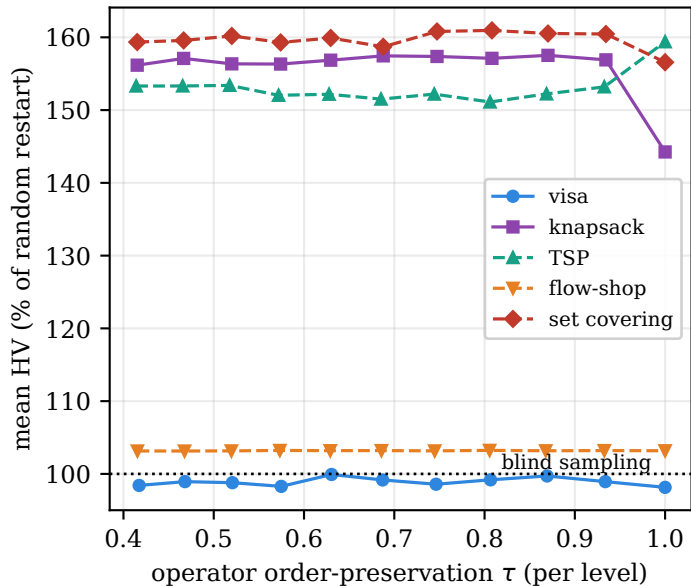
(a) hypervolume
