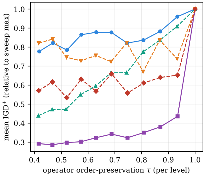
(b) IGD + vs pooled sweep reference
