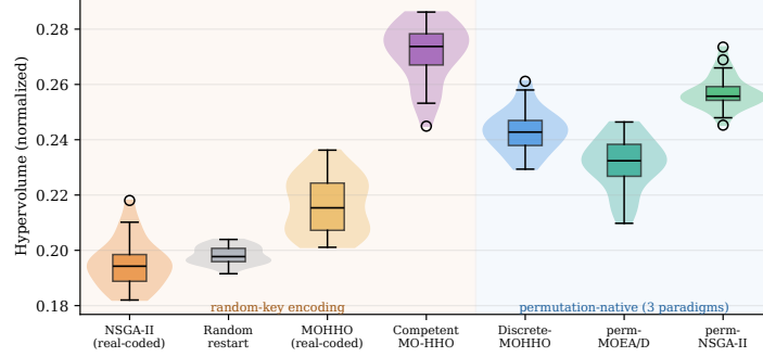
Fig. 10. The seven-method ladder on the multidimensional knapsack (MOMKP), one of the four structures of Table 9. The naive random-key methods (NSGA-II and random restart) sit below the permutation-native methods, while the competent random-key swarm is the single best method here (mean rank 1.13 of seven)—so the divide is non-degenerate search, not the encoding. The split reverses only on the sequencing landscapes (TSP, flow-shop), where the real-coded methods become competitive (Table 9).
