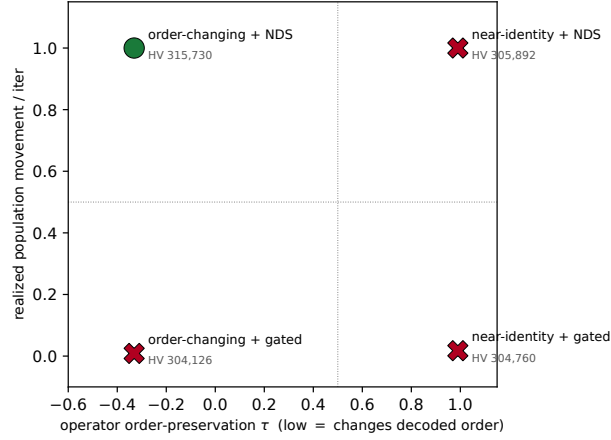
Fig. 8. Mechanism of the two conditions across the 2 \times 2 cells: operator order-preservation \tau (x) versus realized population movement per iteration (y), with each cell’s mean HV annotated. Only the order-changing, diversity-preserving cell occupies the favorable low- \tau , high-movement corner and beats blind sampling.
