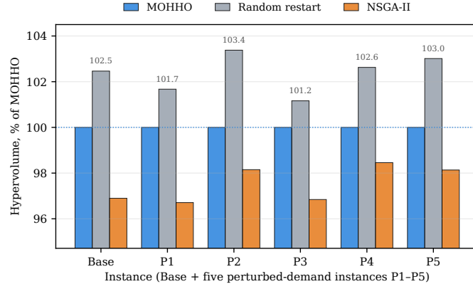
Fig. 9. Generalization over six instances (base plus five \pm 20\% perturbed-demand instances, P1–P5), each method’s mean hypervolume shown as a percentage of MOHHO’s on that instance. The ranking random restart \geq MOHHO > NSGA-II is preserved throughout (101–103 % vs. 96–99 % of MOHHO); on every instance the combined front also dominates the FIFO baseline (not shown).
