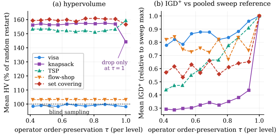
Fig. 7. The registered dose-response sweep: the biased-uniform crossover’s inheritance probability \rho_e swept over eleven levels ( \tau \in [0.42, 1.0] , measured per level) under fixed non-dominated-sorting (NDS) selection, on all five structures (30 seeds per level). (a) Mean hypervolume as a percentage of each structure’s blind random restart (dotted line): every curve is flat in \tau —the four-point sequence in the text is a family contrast, not a dose-response—with the visa below blind sampling throughout (by 0.1–1.9%) and the subset problems (knapsack, set covering) far above it. (b) Mean IGD+ against the pooled sweep front (relative to each structure’s sweep maximum): coverage does degrade as \tau \rightarrow 1 on the visa, knapsack, and TSP—a dose effect the f_2 -dominated hypervolume does not register.
