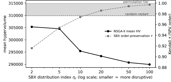
Fig. 6. Sweeping the SBX crossover distribution index \eta_c for the real-coded NSGA-II on the visa problem. As \eta_c falls (more disruptive crossover) the operator order-preservation \tau drops, yet the mean hypervolume never reaches blind random restart (dashed), let alone the permutation tier (dotted); \tau and HV move in strictly opposite directions across the sweep. SBX reaches at most \tau = 0.92 ; the biased-uniform crossover ( \tau = 0.63 ) and HHO moves ( \tau \approx 0 ) extend the operator comparison in Section 6.4.
