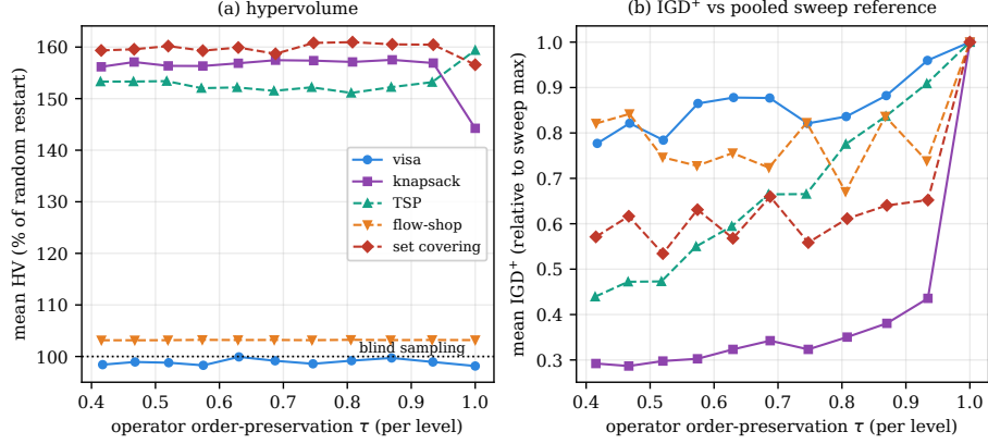
Fig. 7. The registered dose-response sweep: the biased-uniform crossover’s inheritance probability \rho_e swept over eleven levels ( \tau \in [0.42, 1.0] , measured per level) under fixed NDS selection, on all five structures (30 seeds per level). (a) Mean hypervolume as a percentage of each structure’s blind random restart (dotted line): every curve is flat in \tau —the four-point sequence in the text is a family contrast, not a dose-response—with the visa below blind sampling throughout (by 0.1–1.9%) and the subset problems (knapsack, set covering) far above it. (b) Mean IGD + against the pooled sweep front (relative to each structure’s sweep maximum): coverage does degrade as \tau \rightarrow 1 on the visa, knapsack, and TSP—a dose effect the f_2 -dominated hypervolume does not register.
