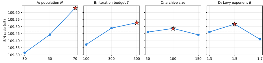
Fig. 1. Main-effects plot of the S/N ratio. The dashed line is the grand mean (109.46 dB) and the red star the best level per factor. Population and iteration budget show clear trends (population the steeper); archive size and \beta are essentially flat.
