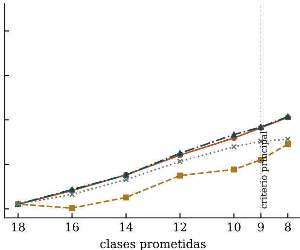
xgb-alphaearth
