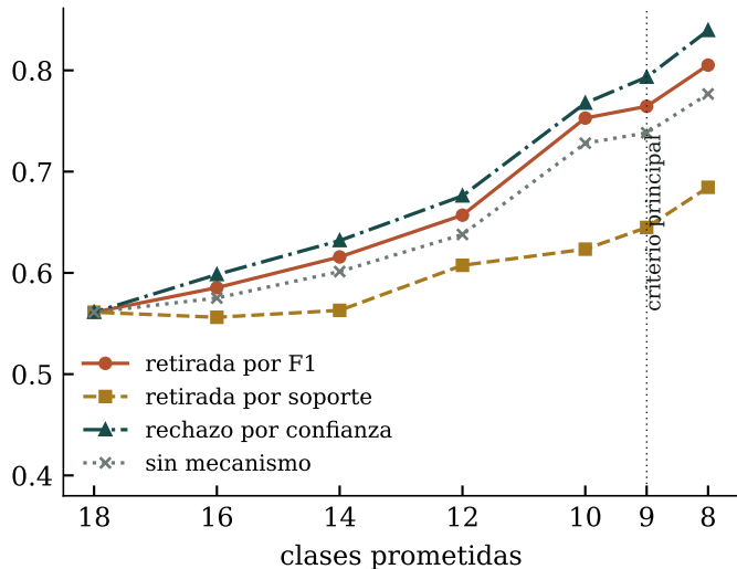
tsvit-pheno
