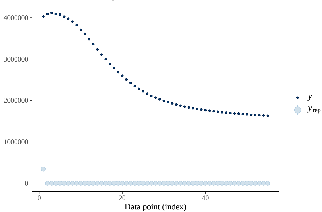
PPC: random walk q – biomass timeseries
