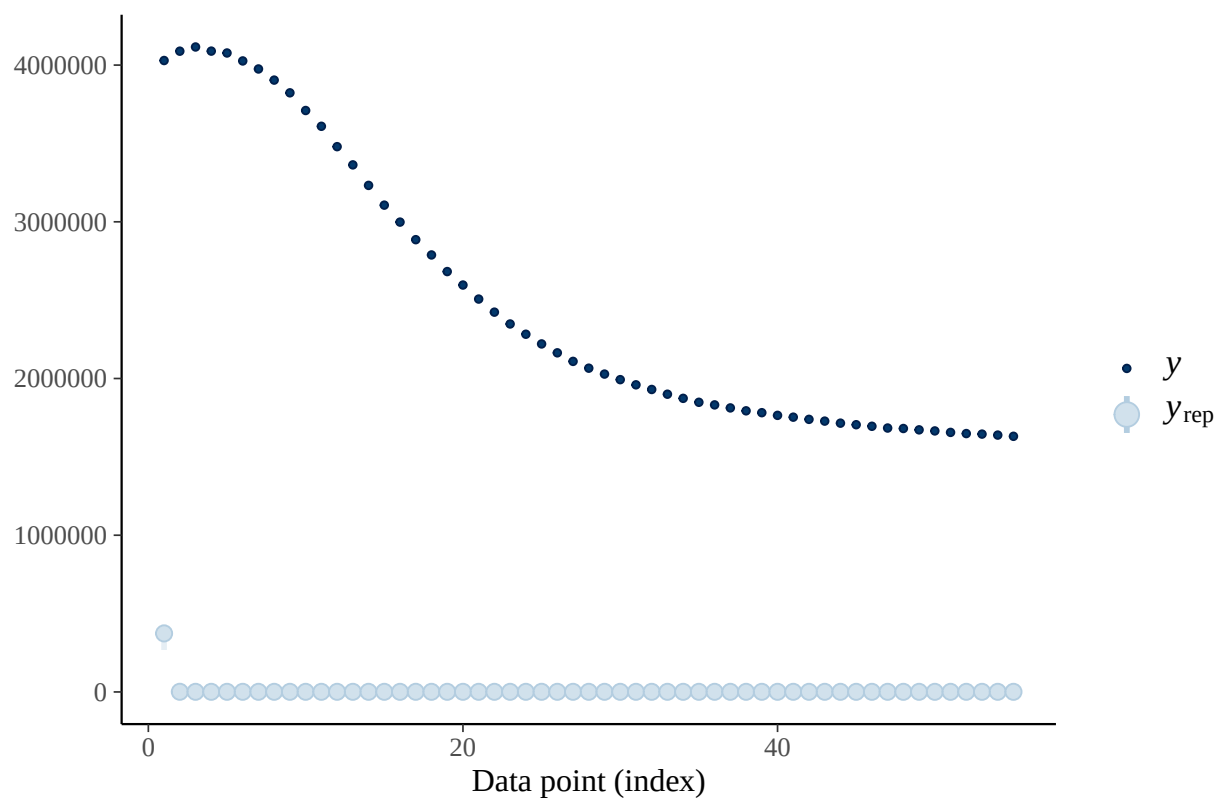
PPC: constant q – biomass timeseries
