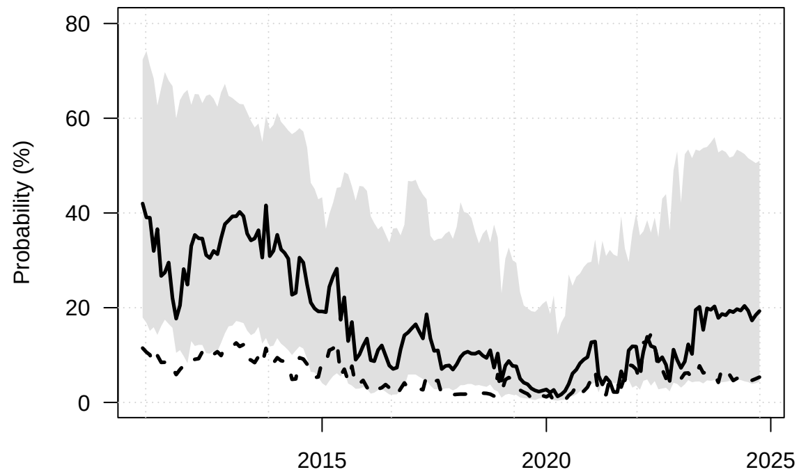
U.S., \pi > 4\%
