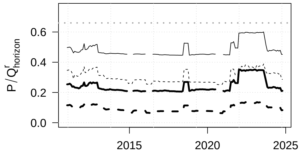
Euro area, \pi > 5\%
