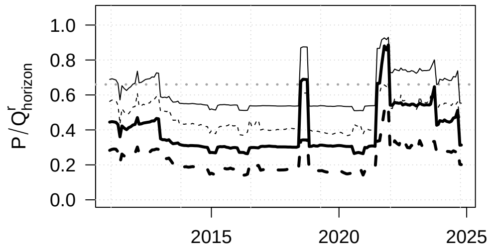
Euro area, \pi > 4\%
