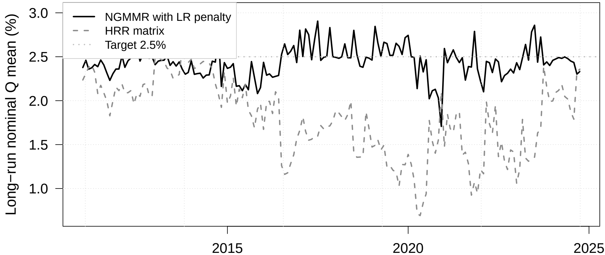
EZ long-run nominal Q mean
