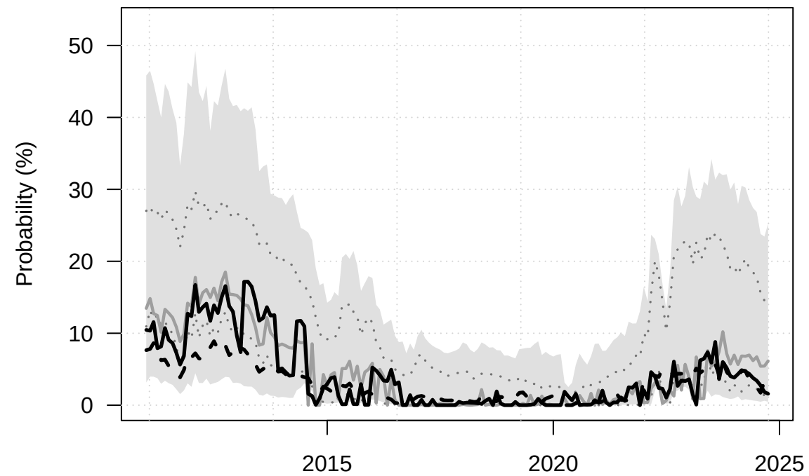
Euro area, \pi_i > 5\%
