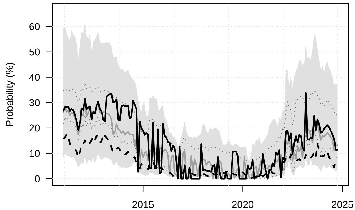
Euro area, \pi_i > 4\%
