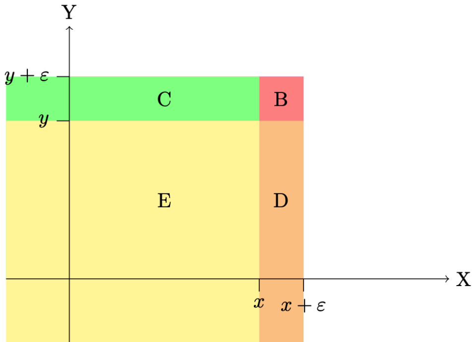
Figure 1.3: Area B+C+D+E encompasses the points with coordinates (X, Y) such that X \leq x+\varepsilon and Y \leq y+\varepsilon . Area D+E encompasses the points with coordinates (X, Y) such that X \leq x+\varepsilon and Y \leq y . Area C+E encompasses the points with coordinates (X, Y) such that X \leq x and Y \leq y+\varepsilon .
