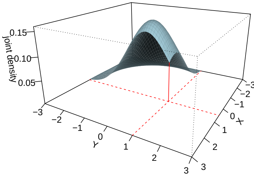
Figure 1.1: The volume between the horizontal plane ( z = 0 ) and the surface is equal to F_{XY}(0.5, 1) = \mathbb{P}(X < 0.5, Y < 1) .
