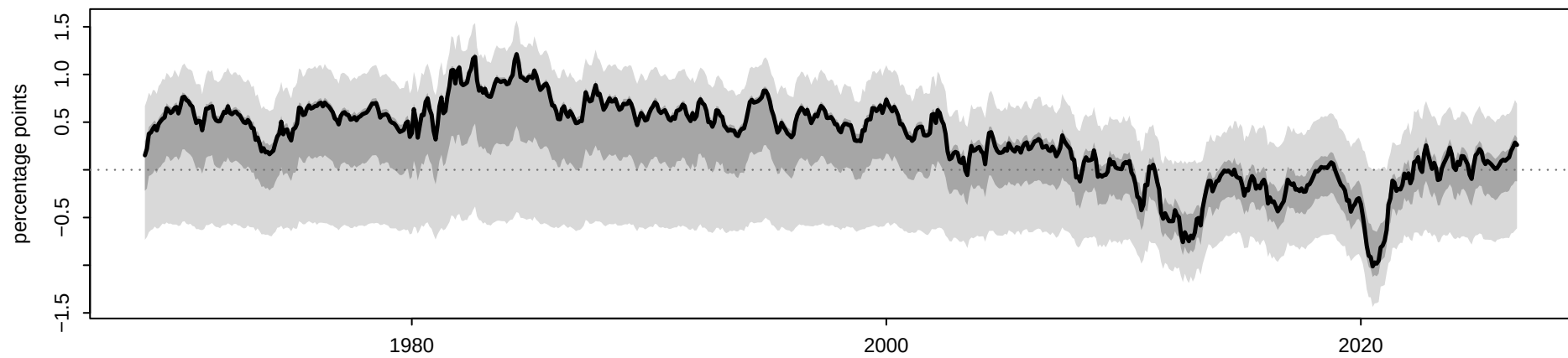
(c) 10-year inflation risk premium
