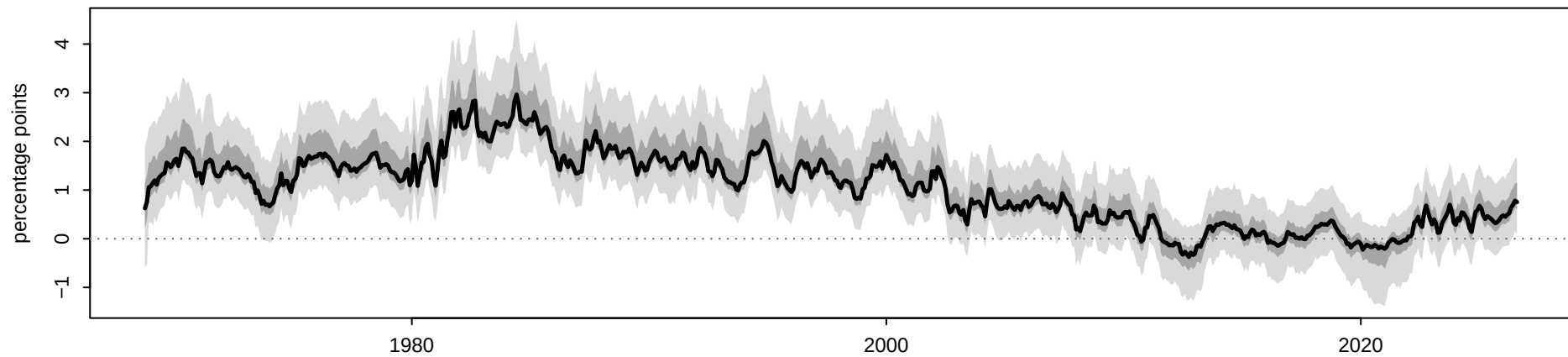
(b) 10-year real term premium
