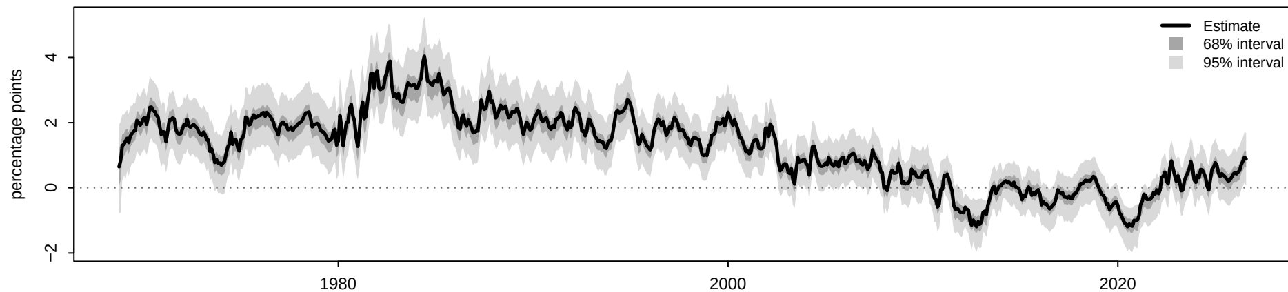
(a) 10-year nominal term premium
