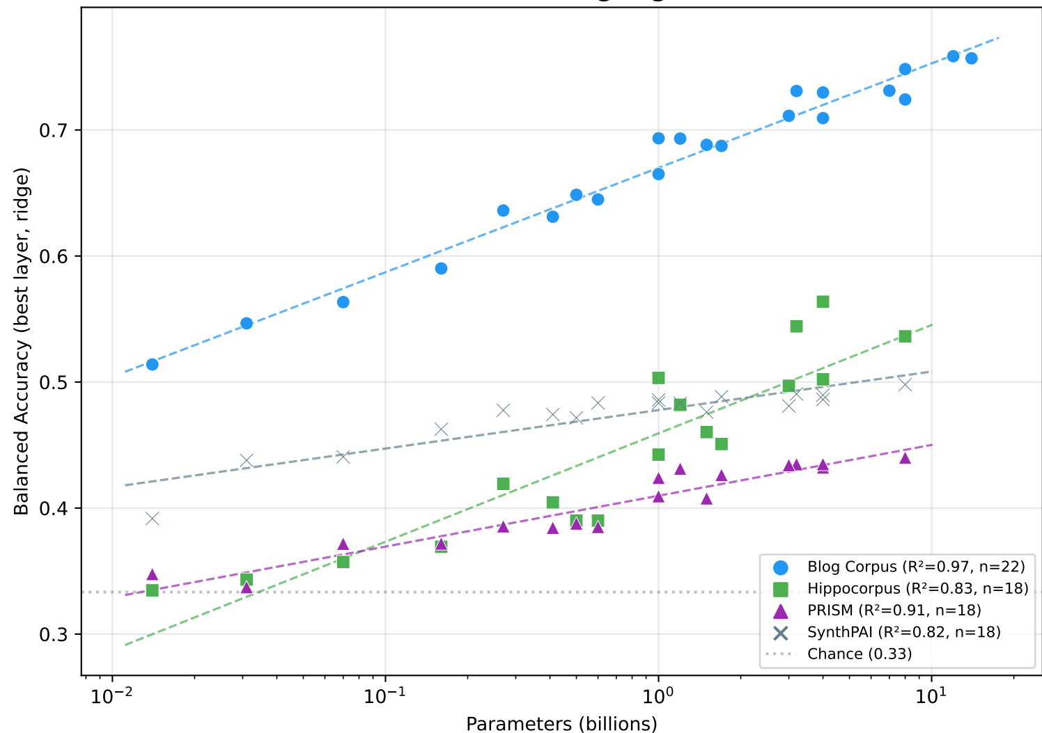
Cross-Dataset Scaling: Age (3-class)
