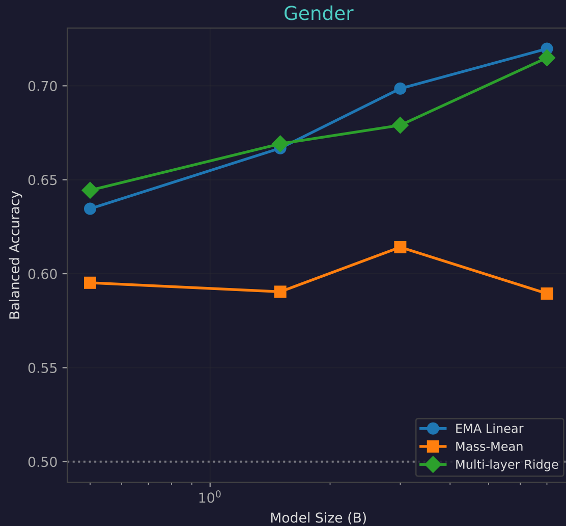
Scaling Curve: Probe Accuracy vs Model Size
