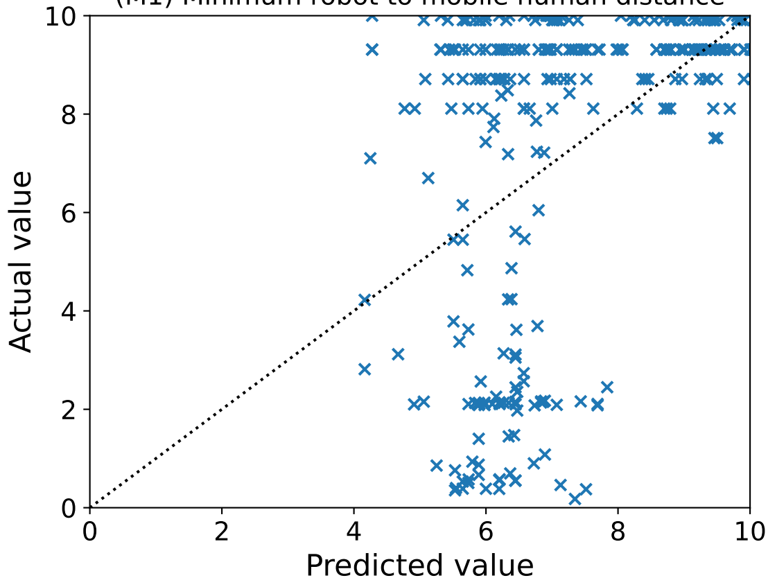
(M1) Minimum robot to mobile human distance
