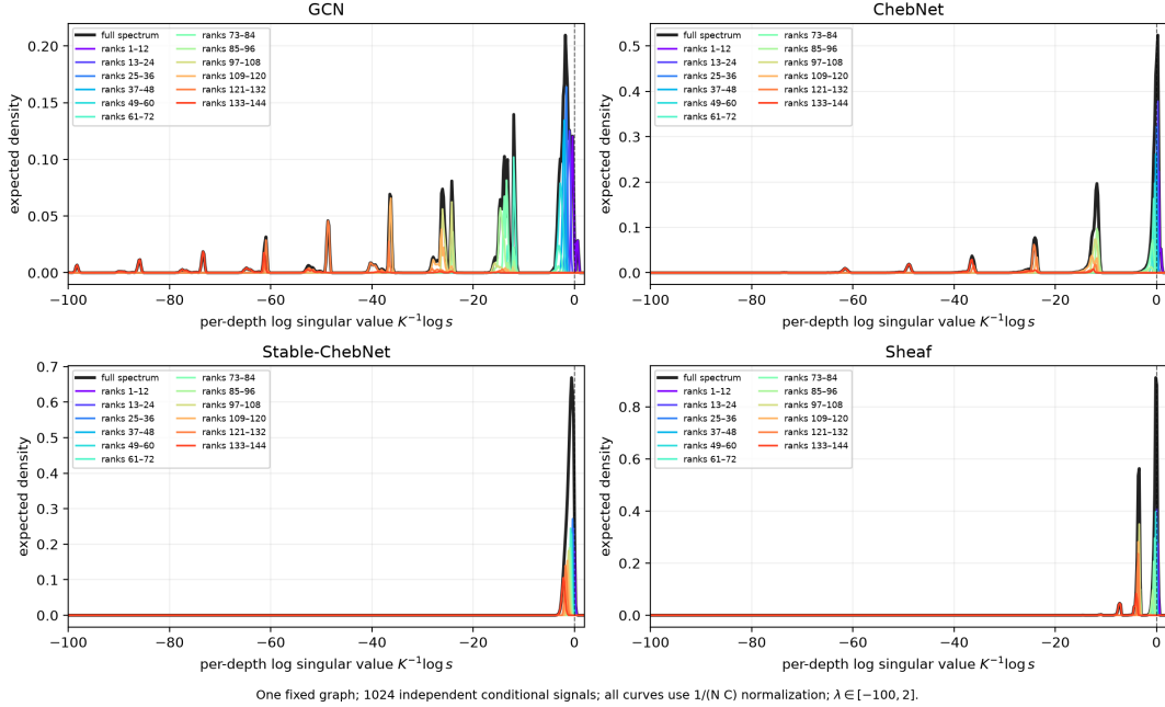
Fixed-graph conditional channel-grouped expected empirical measures
