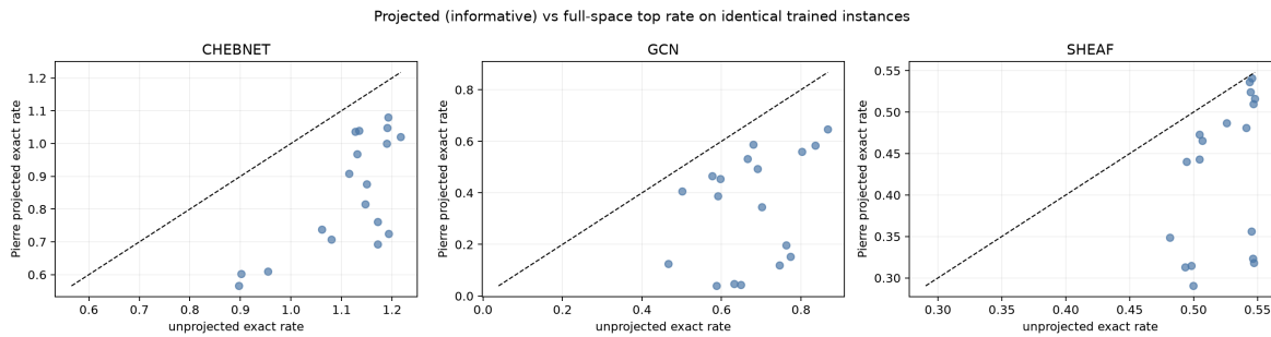
Figure 17. Projection lowers the measured top rate on these matched cells, but the projected quantity remains positive on average. The comparison is between two estimands, not two implementations of one estimator.
