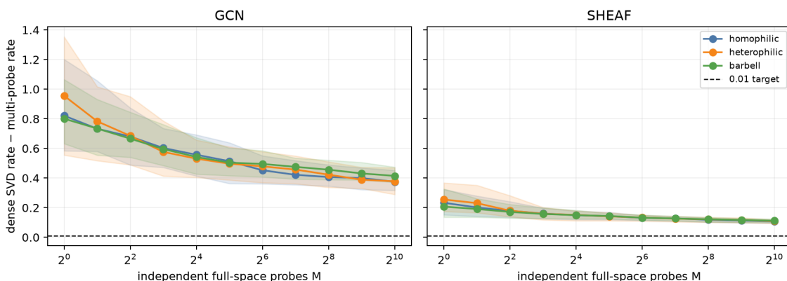
Random-probe lower-bound convergence by architecture and graph family
