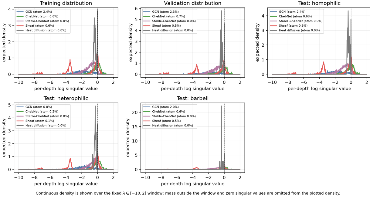
Figure 14. Expected empirical log-singular-value density on a linear y-axis with a fixed \lambda \in [-10, 2] window. The full tangent-space normalization is retained, so mass outside the window and the -\infty atom are omitted from the displayed density.
