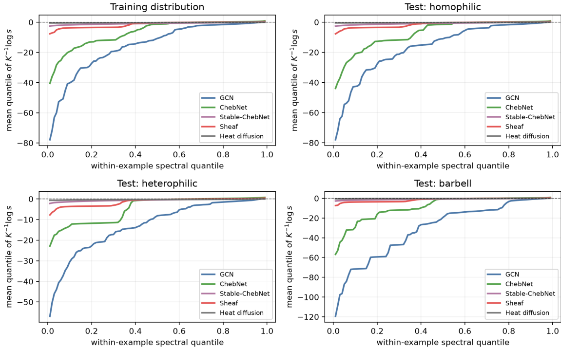
Figure 15. Mean within-example spectral quantile profiles. These curves complement the expected CDFs and PDFs and show how the bulk, not only the top mode, changes across systems and graph families.
