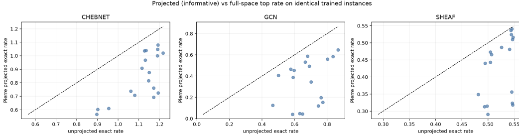
Figure 9. Projection lowers the measured top rate on these matched cells, but the projected quantity remains positive on average. The comparison is between two estimands, not two implementations of one estimator.
