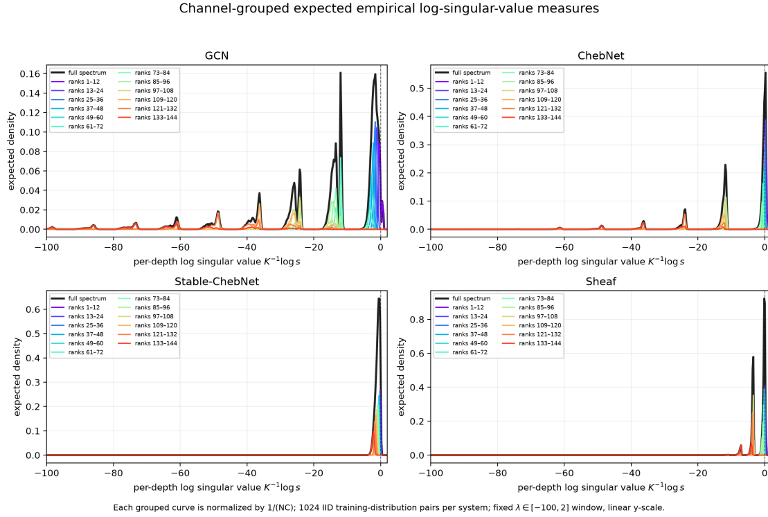
Figure 18. Full and all-twelve-channel-grouped expected empirical densities for GCN, ChebNet, Stable-ChebNet, and sheaf. The solid black curve is the full spectrum; the twelve colored curves cycle through a rainbow palette for ranks 1-12, 13-24, ..., and 133-144. Every curve uses 1/(NC) normalization, so each grouped measure has mass 1/N before truncation.
