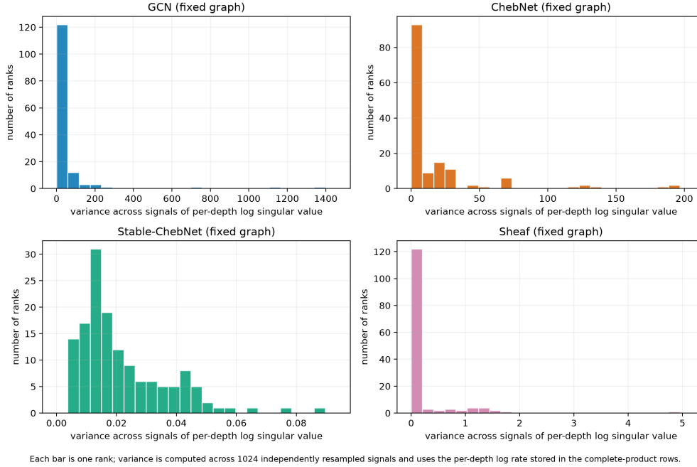
Figure 18b. Histograms of the rank-wise variance of per-depth log singular values across the 1,024 fixed-graph signal realizations, one panel per architecture. Each bar is one of the 144 descending singular-value ranks; zero-singular-value occurrences are excluded from the per-rank variance and their finite fractions are recorded in the evidence summary.
