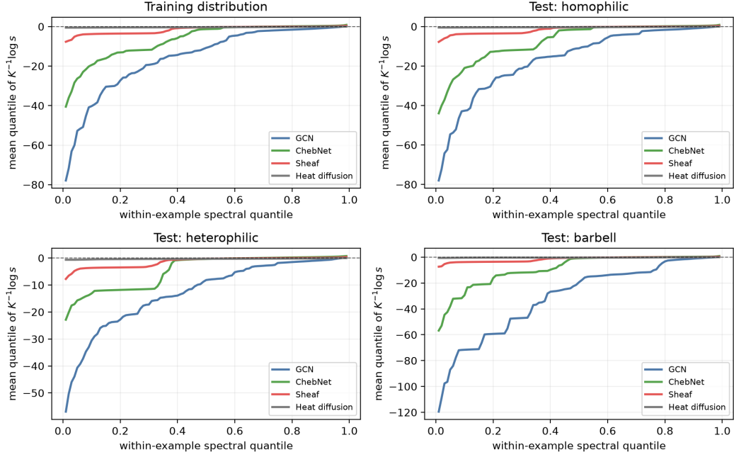
Figure 10. Mean within-example spectral quantile profiles. These curves complement the expected CDFs and show how the bulk, not only the top mode, changes across systems and graph families.
