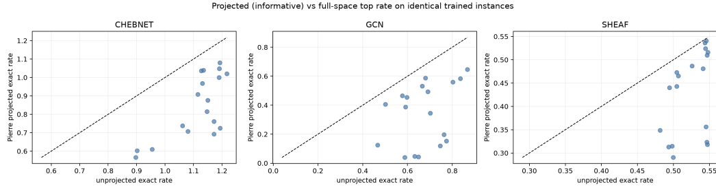
Figure 11. Projection lowers the measured top rate on these matched cells, but the projected quantity remains positive on average. The comparison is between two estimands, not two implementations of one estimator.
