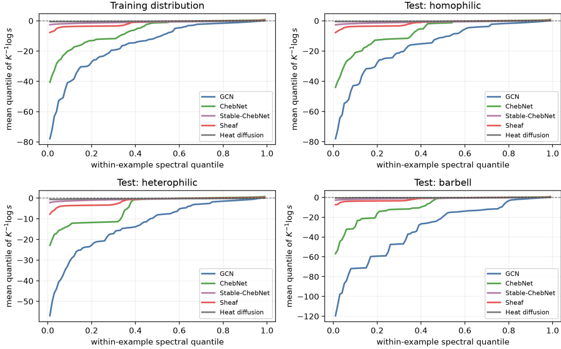
Figure 16. Mean within-example spectral quantile profiles. These curves complement the expected CDFs and PDFs and show how the bulk, not only the top mode, changes across systems and graph families.
