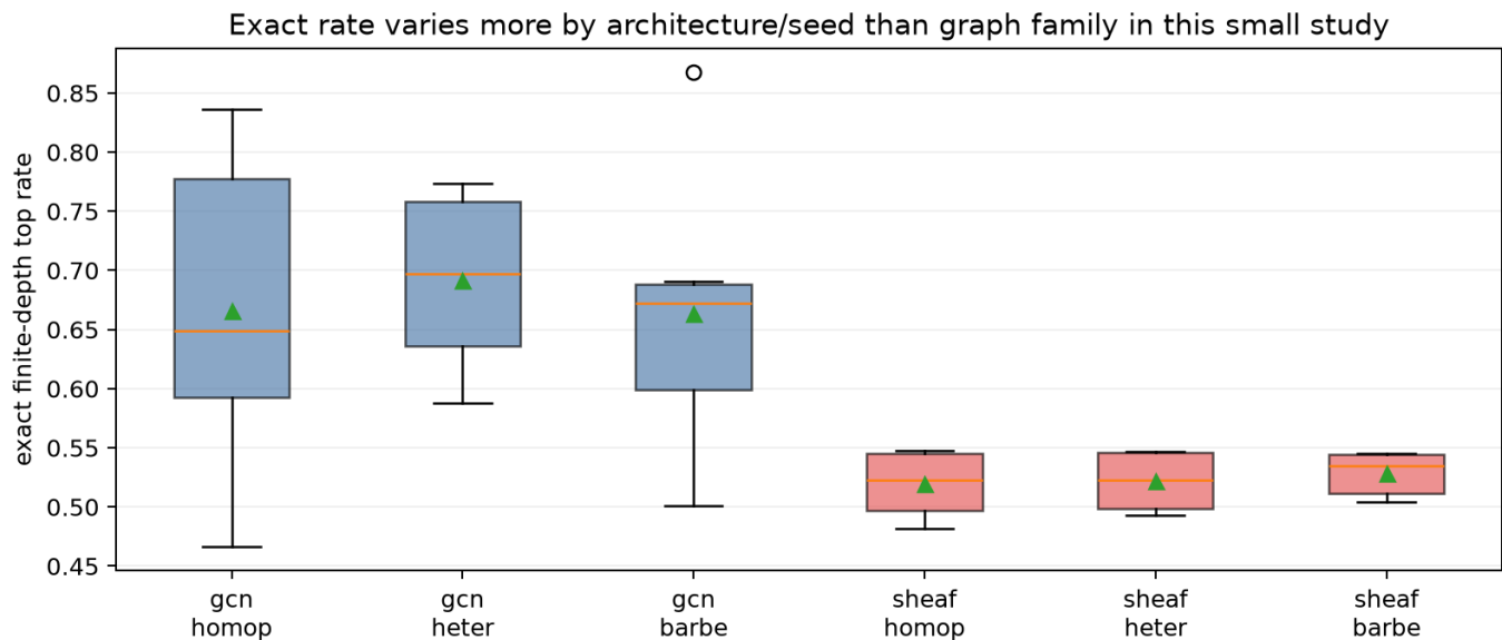
Figure 7: Exact-rate distribution
