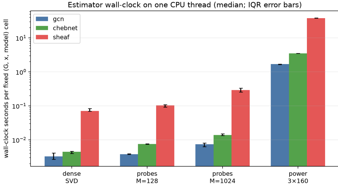
Figure 9: Estimator wall-clock comparison
