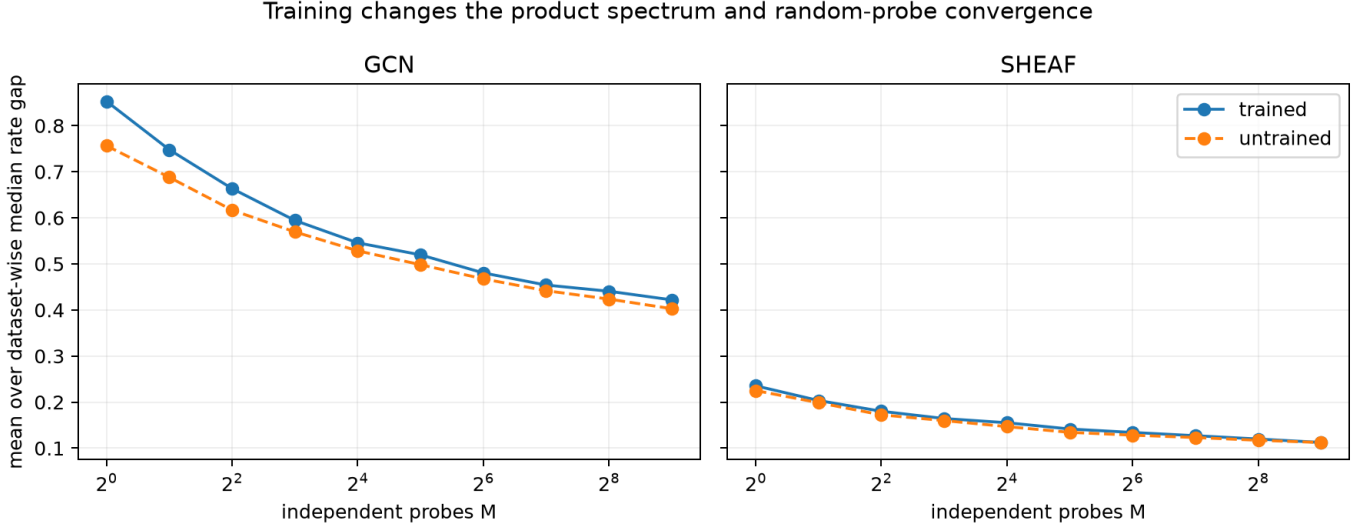
Figure 8: Training-state probe comparison
