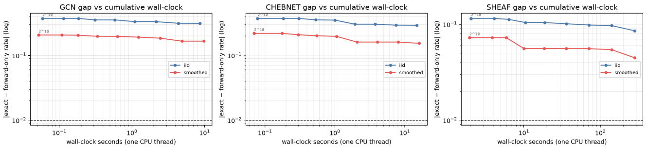
Best forward-only estimator wall-clock Pareto (forward probes only; rightmost point = M = 2^{20} )
