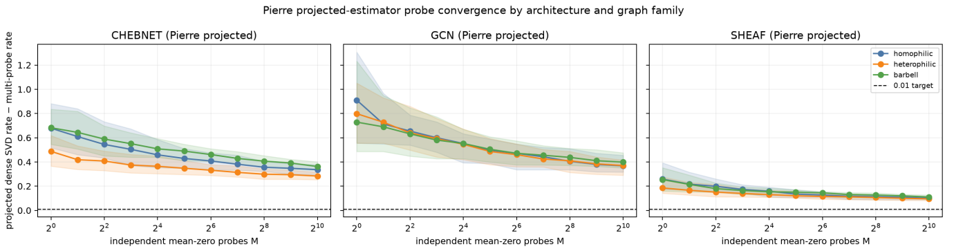
Figure 11: Pierre projected-probe convergence
