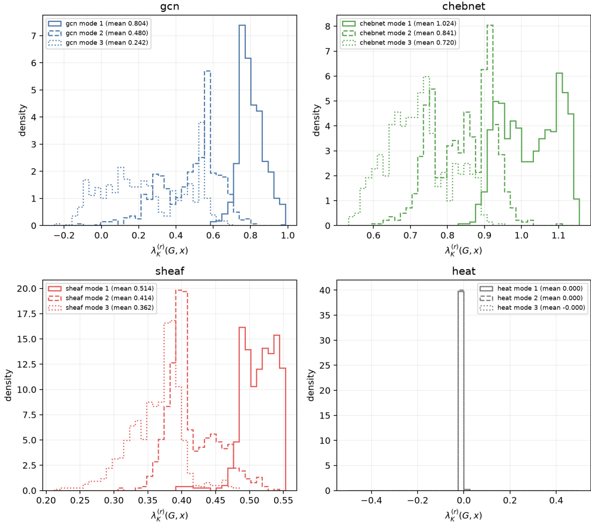
Figure 9: Finite-depth eigenmode rate histograms per system
