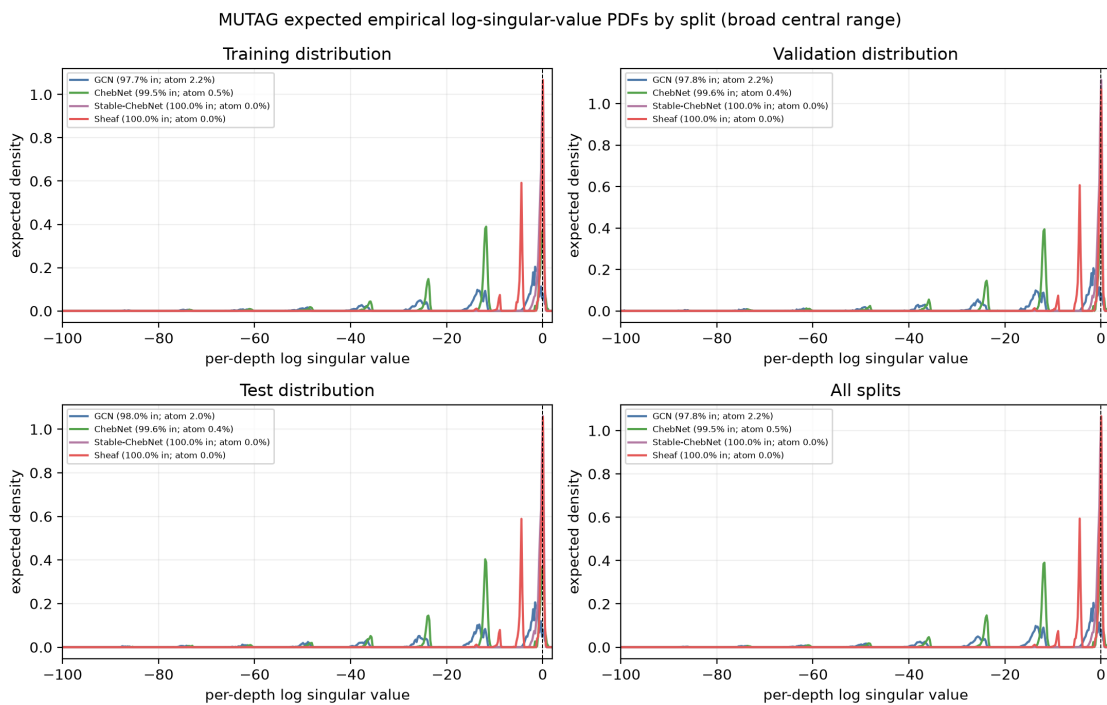
Figure 24. MUTAG split-wise expected empirical log-singular-value PDFs over a data-derived broad central finite-rate range, analogous to Figure 12. Each panel compares all four trained architectures and annotates finite-window and atom mass.
