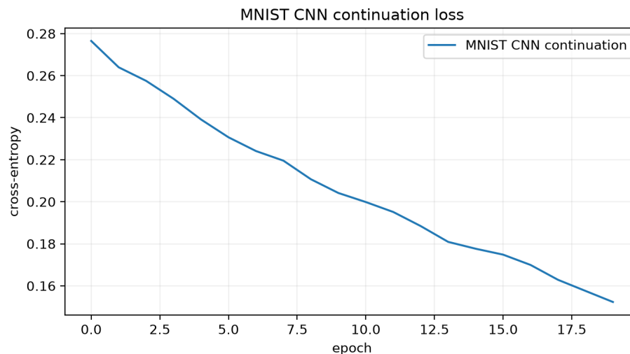
Figure 36. MNIST CNN continuation loss. The initial and continued validation accuracies, exact JVP/reverse-mode agreement, source-state hashes, and sampled-image provenance are recorded in the continuation evidence summary.
