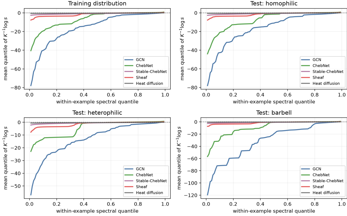
Figure 14. Mean within-example spectral quantile profiles. These curves complement the expected CDFs and PDFs and show how the bulk, not only the top mode, changes across systems and graph families.
