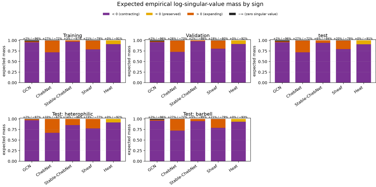
Figure 15. Expected empirical-measure mass by sign for every architecture and distribution. Labels show positive/negative finite-rate mass; the stacked bars additionally show exact zero-rate mass and the -\infty zero-singular-value atom.
