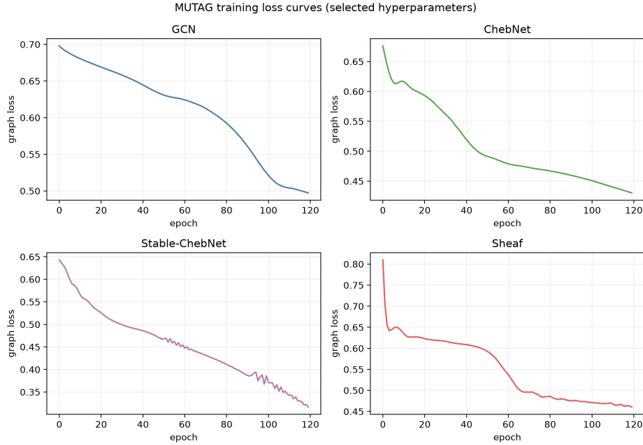
Figure 30. MUTAG graph-classification loss curves for the selected learning-rate candidate of each architecture.
