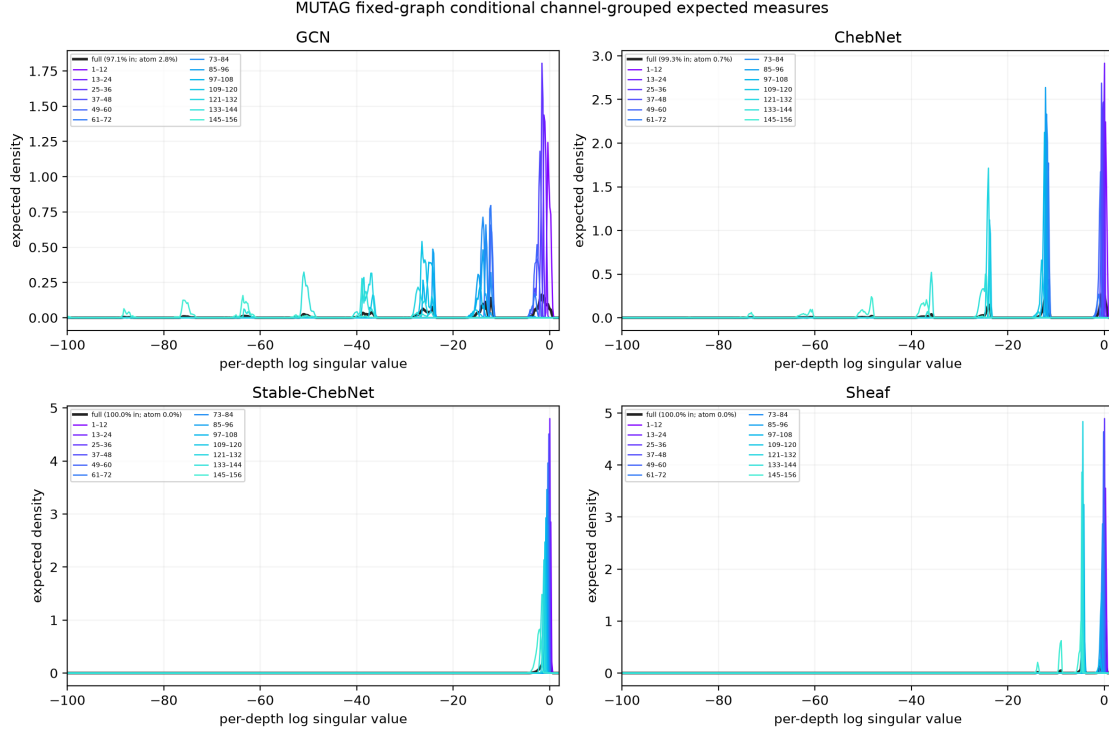
Figure 29. MUTAG fixed-graph conditional channel-grouped expected measures, analogous to the fixed-graph Figure 18a. One training graph is held fixed while 256 independent feature-noise signals are sampled; the number of channel-sized rank groups is determined by that graph's node count.
