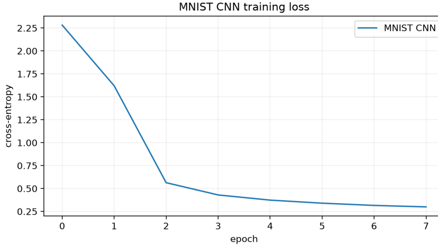
Figure 33. MNIST CNN training loss. The validation accuracy and exact JVP/reverse-mode agreement are recorded in the evidence summary.
