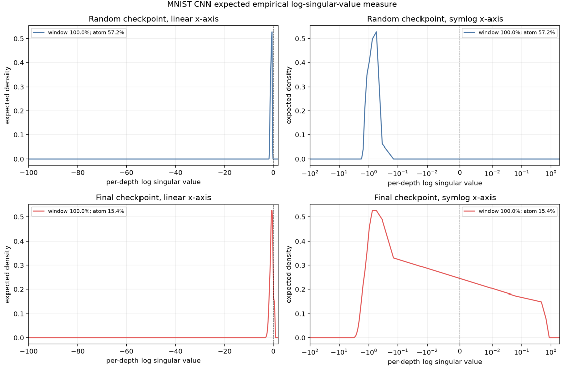
Figure 32. MNIST CNN expected empirical log-singular-value densities. The top row is the random initialization and the bottom row is the final checkpoint; columns show linear and symmetric-log horizontal axes. Each curve averages per-image empirical measures with full hidden-state normalization.
