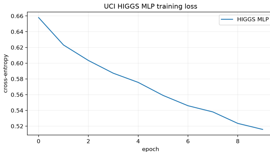
Figure 35. UCI HIGGS MLP training loss. The bounded subset, validation gate, random sampling seed and model provenance are recorded in the evidence manifest.
