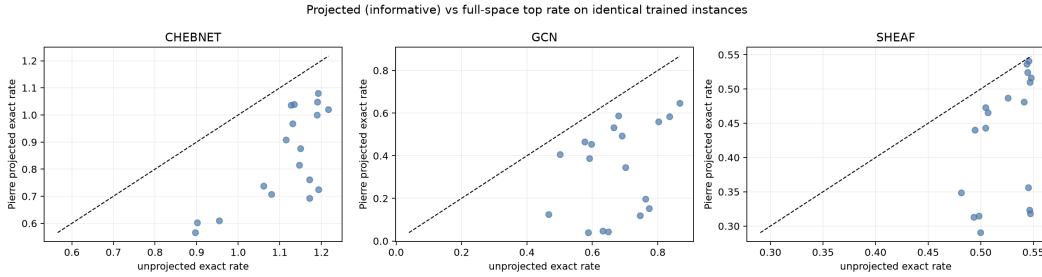
Figure 31. Projection lowers the measured top rate on these matched cells, but the projected quantity remains positive on average. The comparison is between two estimands, not two implementations of one estimator.
