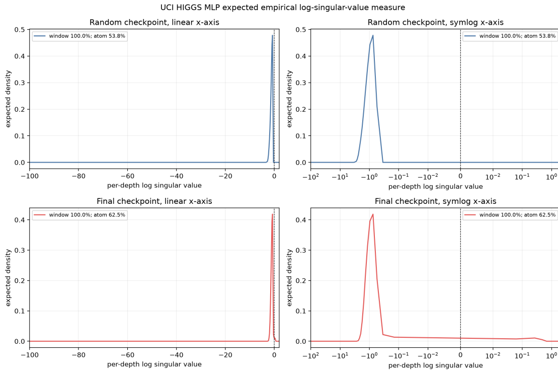
Figure 34. UCI HIGGS four-hidden-layer 300-unit MLP expected empirical log-singular-value densities, with random and final checkpoints in the top and bottom rows and linear/symmetric-log horizontal axes in the columns.
