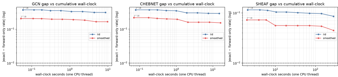
Figure 8. Gap versus cumulative wall-clock for iid and graph-smoothed forward-only probes. Probe work is batched; the total wall-clock still grows with M , especially for the deep sheaf.
