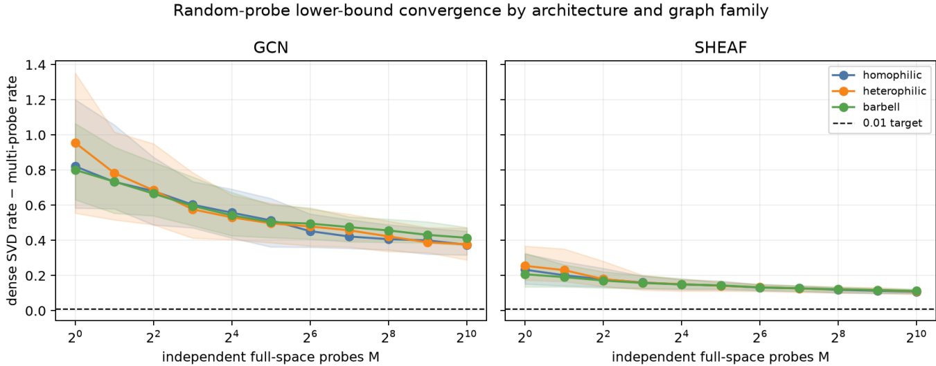
Figure 2: Probe convergence summary
