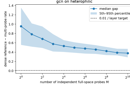
GCN heterophilic
