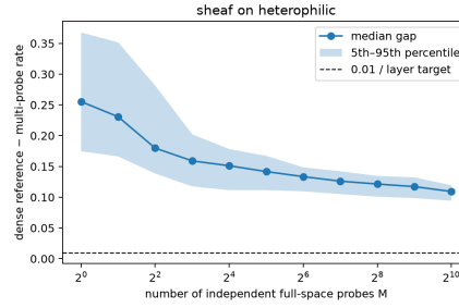
Sheaf heterophilic
