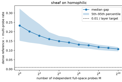
Sheaf homophilic
