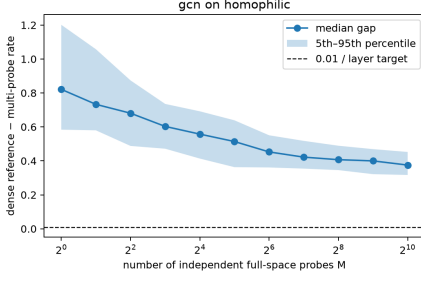
GCN homophilic
