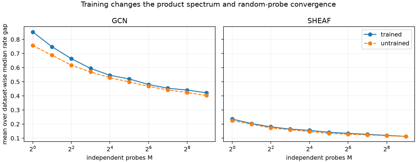
Figure 5: Training-state probe comparison
