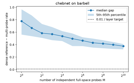
ChebNet barbell
