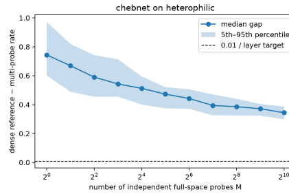
ChebNet heterophilic
