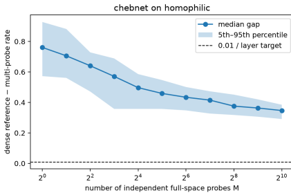
ChebNet homophilic
