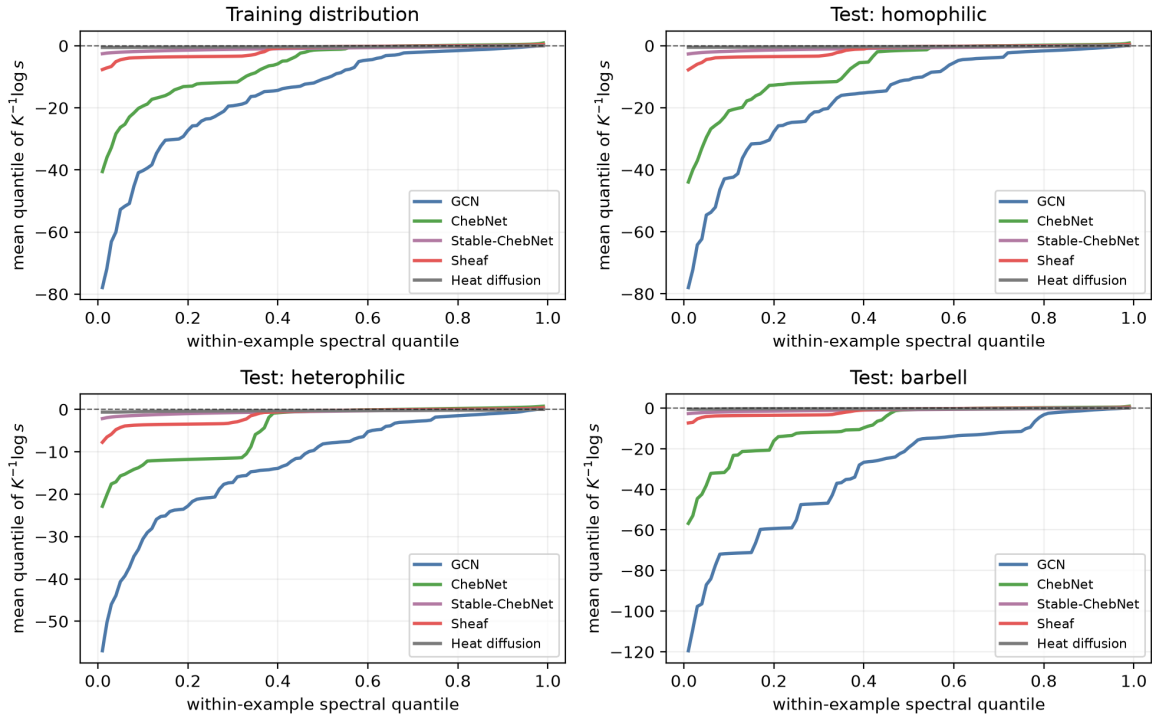
Figure 19. Mean within-example spectral quantile profiles. These curves complement the expected CDFs and PDFs and show how the bulk, not only the top mode, changes across systems and graph families.
