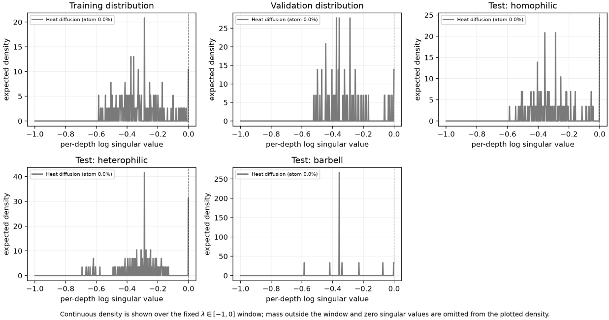
Figure 15. Heat-diffusion expected empirical density zoomed to \lambda \in [-1, 0] on a linear y-axis. The five panels are the training, validation, and three test distributions; only heat diffusion is plotted.
