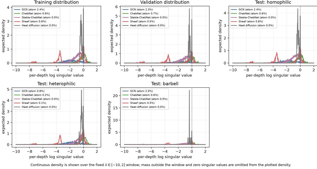
Figure 14. Expected empirical log-singular-value density on a linear y-axis with a fixed \lambda \in [-10, 2] window. The full tangent-space normalization is retained, so mass outside the window and the -\infty atom are omitted from the displayed density.
