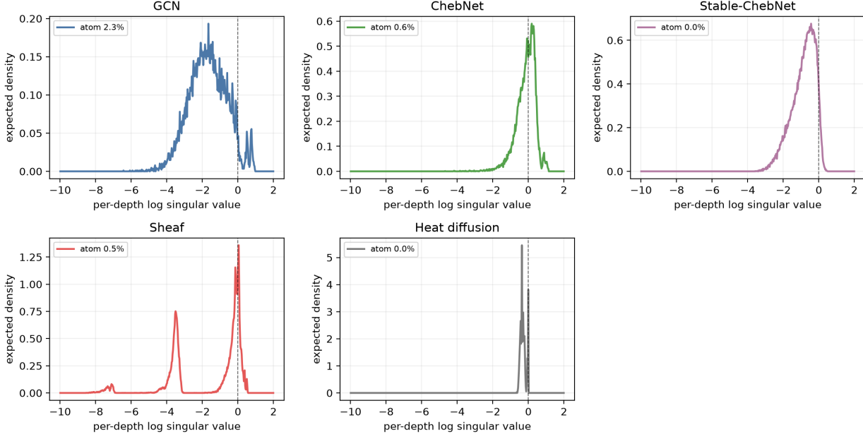
Figure 16. Expected empirical log-singular-value PDFs on the training distribution using 256 independent graph-signal pairs per system, one panel per architecture/dynamical system. The fixed \lambda \in [-10, 2] window and linear y-axis match Figure 14; each curve retains full tangent-space normalization.
