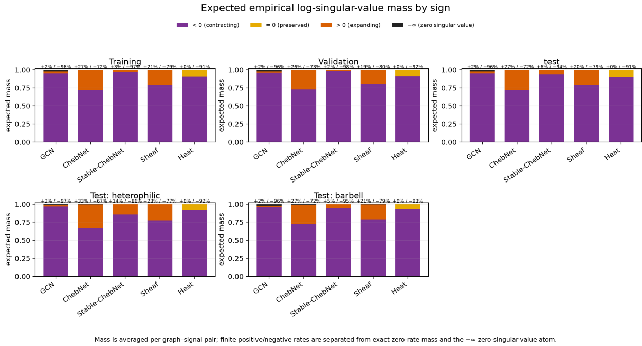
Figure 20. Expected empirical-measure mass by sign for every architecture and distribution. Labels show positive/negative finite-rate mass; the stacked bars additionally show exact zero-rate mass and the -\infty zero-singular-value atom.
