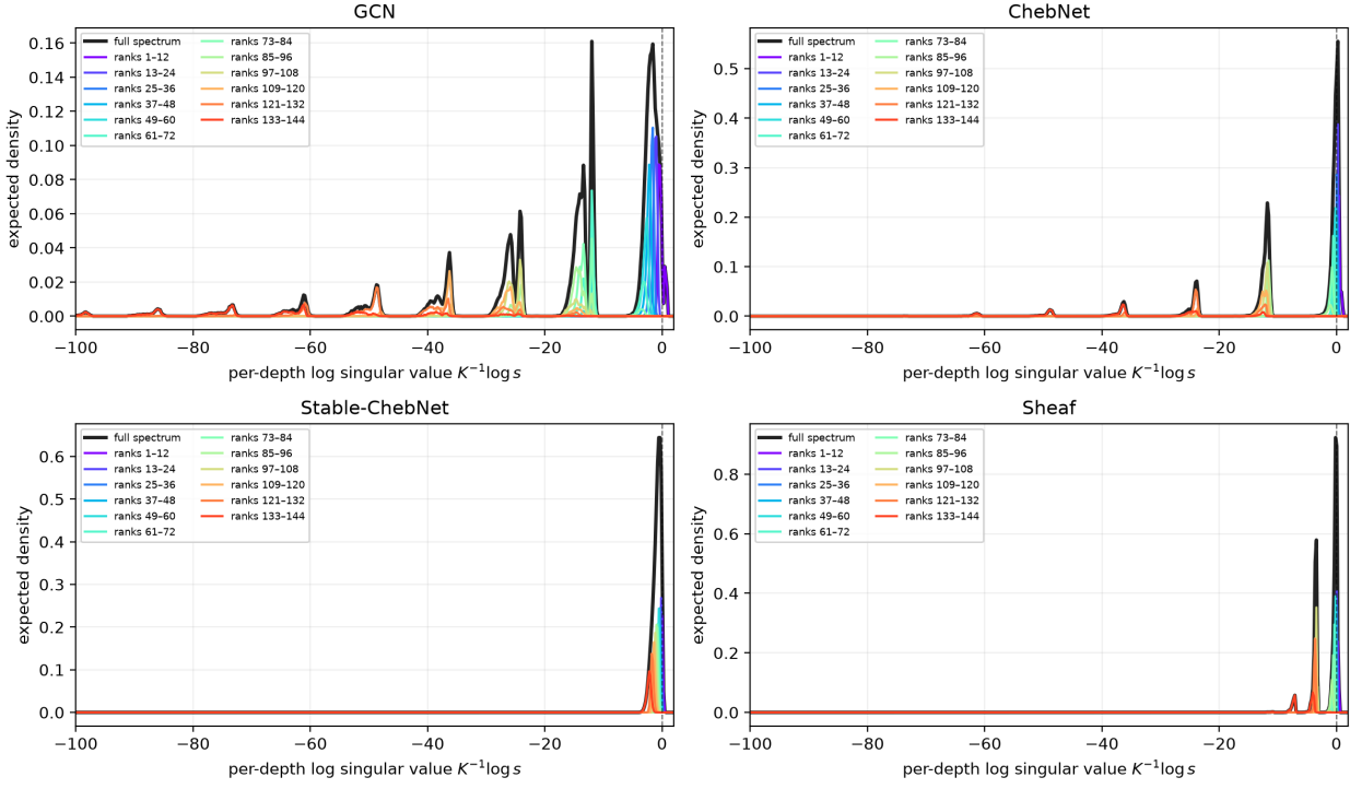
Figure 18. Full and all-twelve-channel-grouped expected empirical densities for GCN, ChebNet, Stable-ChebNet, and sheaf. The solid black curve is the full spectrum; the twelve colored curves cycle through a rainbow palette for ranks 1-12, 13-24, ..., and 133-144. Every curve uses 1/(NC) normalization, so each grouped measure has mass 1/N before truncation.
