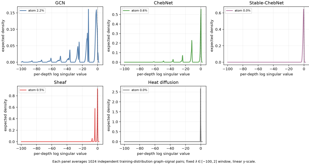
Figure 17. Expected empirical log-singular-value PDFs on the same training distribution using 1024 distinct IID graph-signal pairs per system. The wider fixed \lambda \in [-100, 2] window exposes the far contracting tails while retaining a linear y-axis and full tangent-space normalization.
