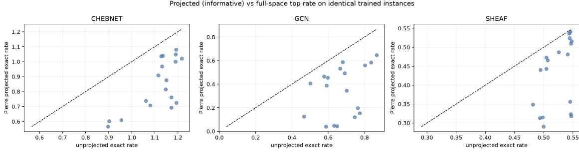
Figure 21. Projection lowers the measured top rate on these matched cells, but the projected quantity remains positive on average. The comparison is between two estimands, not two implementations of one estimator.
