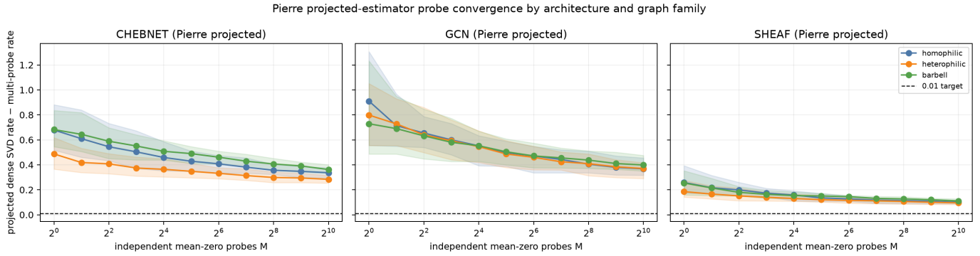
Figure 9: Pierre projected-probe convergence
