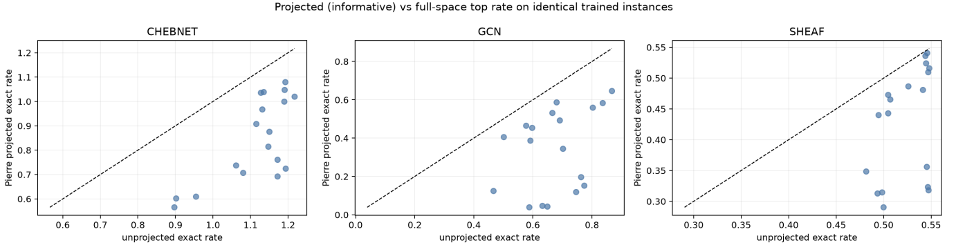
Figure 8: Projected versus unprojected exact rates
