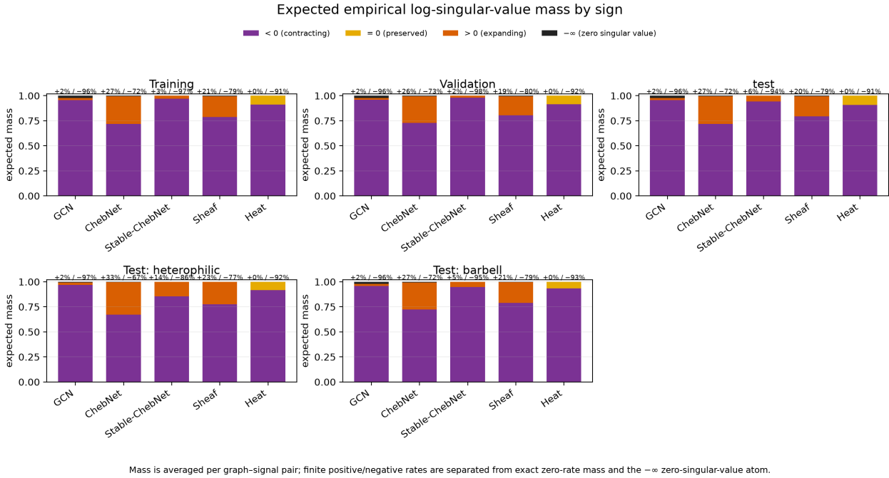
Figure 19. Expected empirical-measure mass by sign for every architecture and distribution. Labels show positive/negative finite-rate mass; the stacked bars additionally show exact zero-rate mass and the -\infty zero-singular-value atom.
