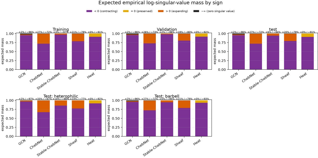
Figure 18. Expected empirical-measure mass by sign for every architecture and distribution. Labels show positive/negative finite-rate mass; the stacked bars additionally show exact zero-rate mass and the -\infty zero-singular-value atom.
