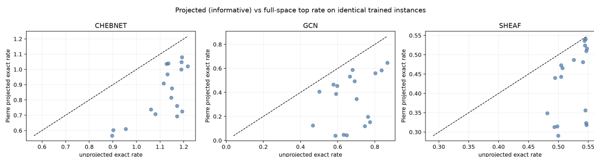
Figure 19. Projection lowers the measured top rate on these matched cells, but the projected quantity remains positive on average. The comparison is between two estimands, not two implementations of one estimator.
