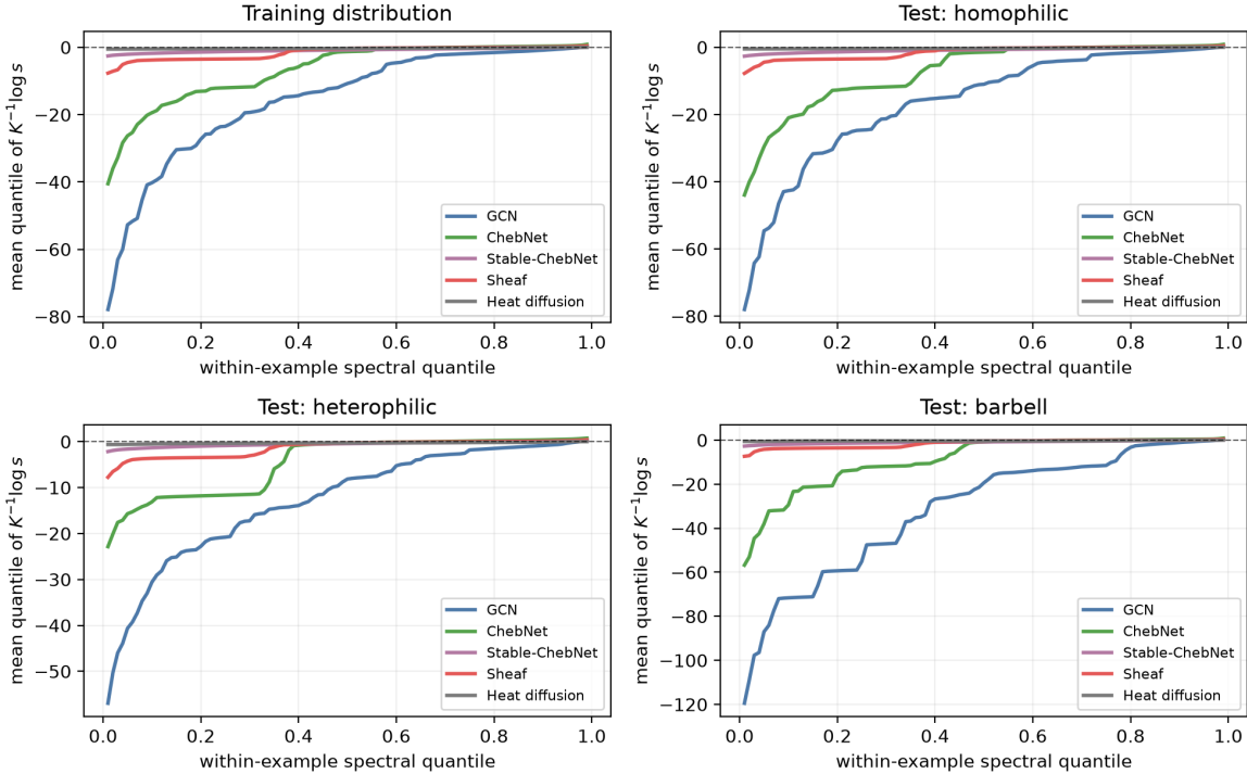
Figure 17. Mean within-example spectral quantile profiles. These curves complement the expected CDFs and PDFs and show how the bulk, not only the top mode, changes across systems and graph families.
