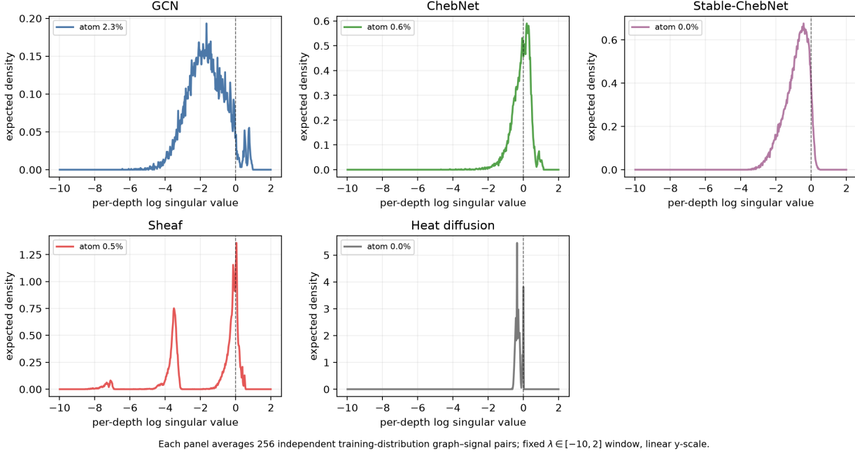
Figure 16. Expected empirical log-singular-value PDFs on the training distribution using 256 independent graph-signal pairs per system, one panel per architecture/dynamical system. The fixed \lambda \in [-10, 2] window and linear y-axis match Figure 14; each curve retains full tangent-space normalization.
