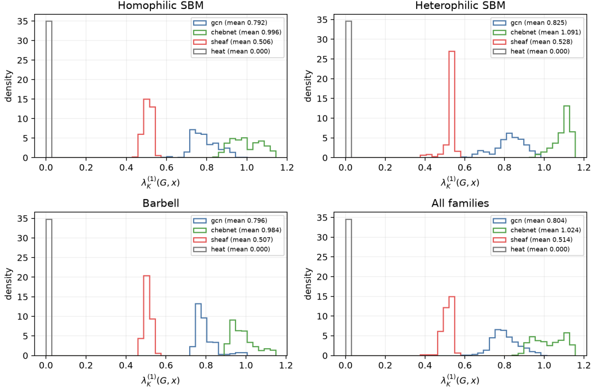
Figure 9: Exact Lyapunov-rate histograms over random (G, x) pairs
