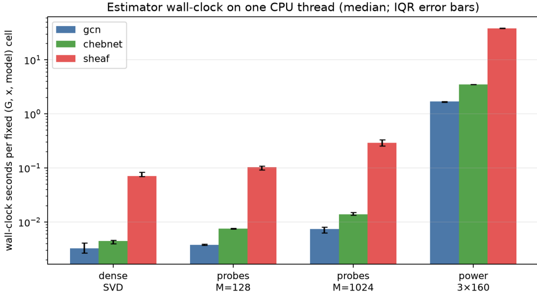
Figure 8: Estimator wall-clock comparison
