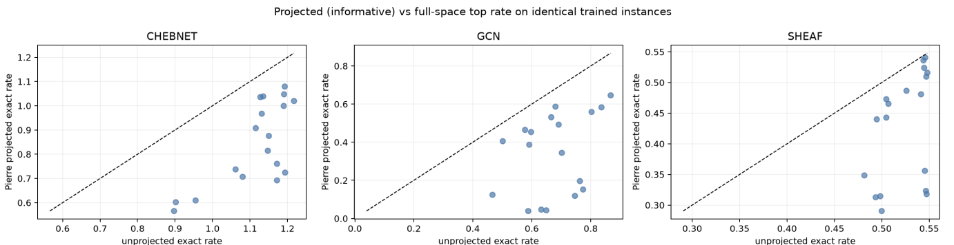
Figure 11: Projected versus unprojected exact rates
