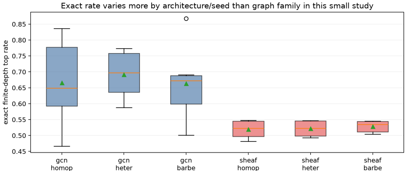
Figure 6: Exact-rate distribution
