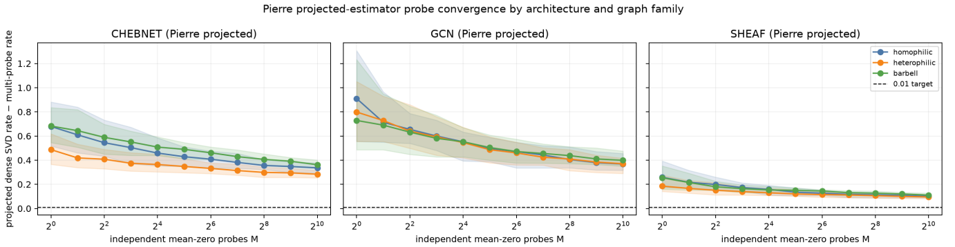
Figure 12: Pierre projected-probe convergence
