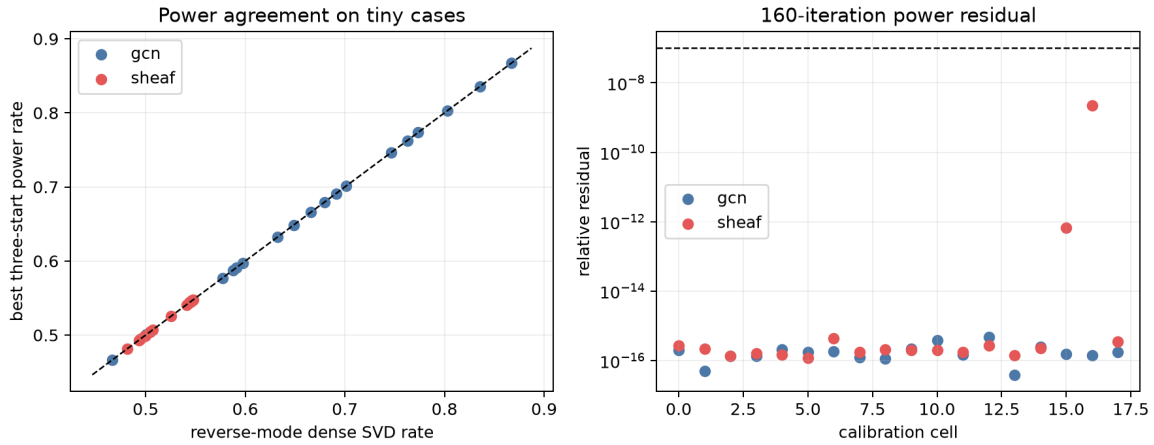
Figure 5: Power versus exact SVD
