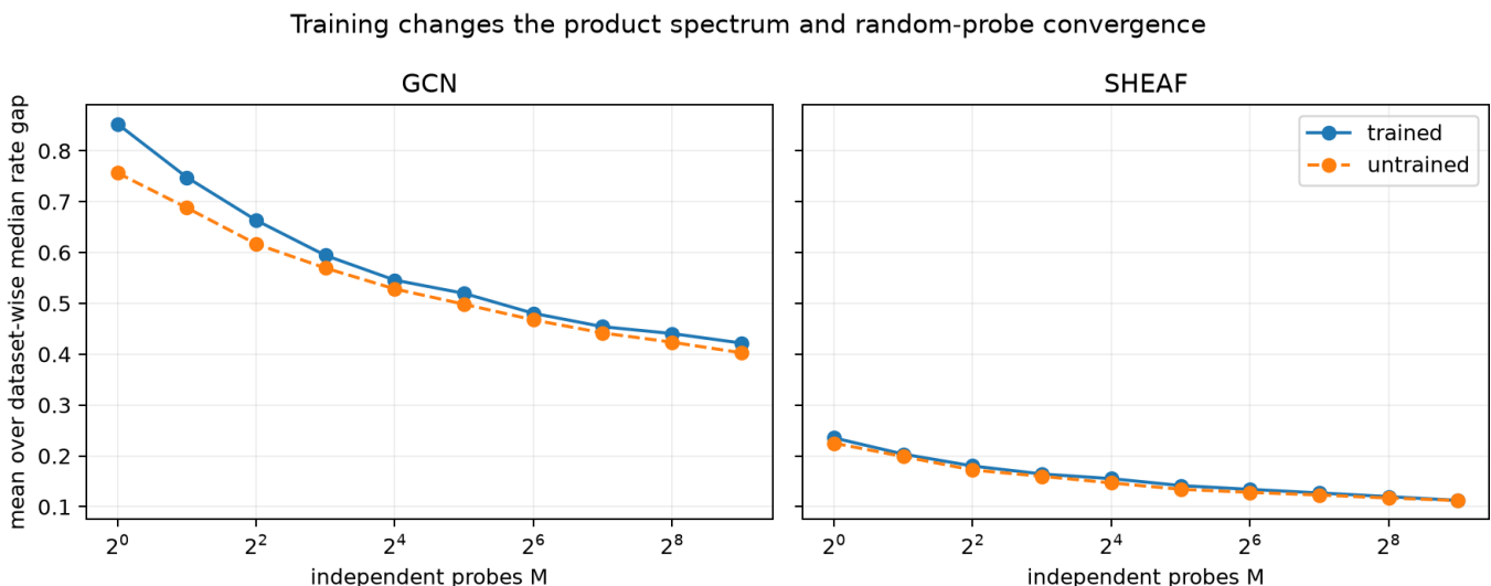
Figure 7: Training-state probe comparison
