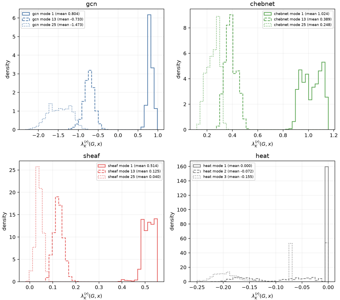
Figure 10: Finite-depth eigenmode rate histograms per system
