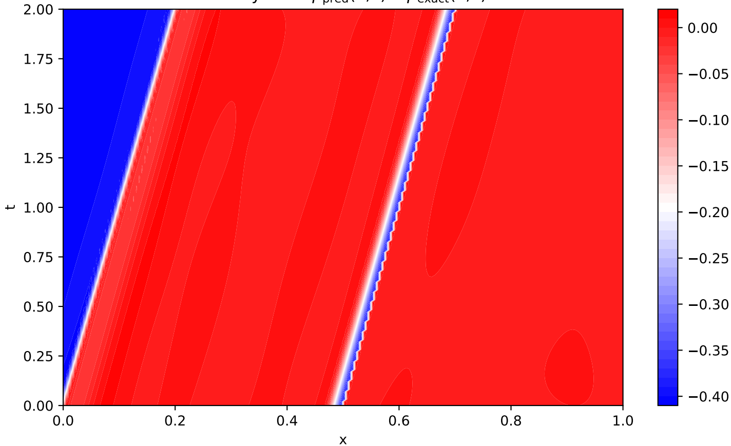
Density error \rho_{\text{pred}}(x, t) - \rho_{\text{exact}}(x, t)
