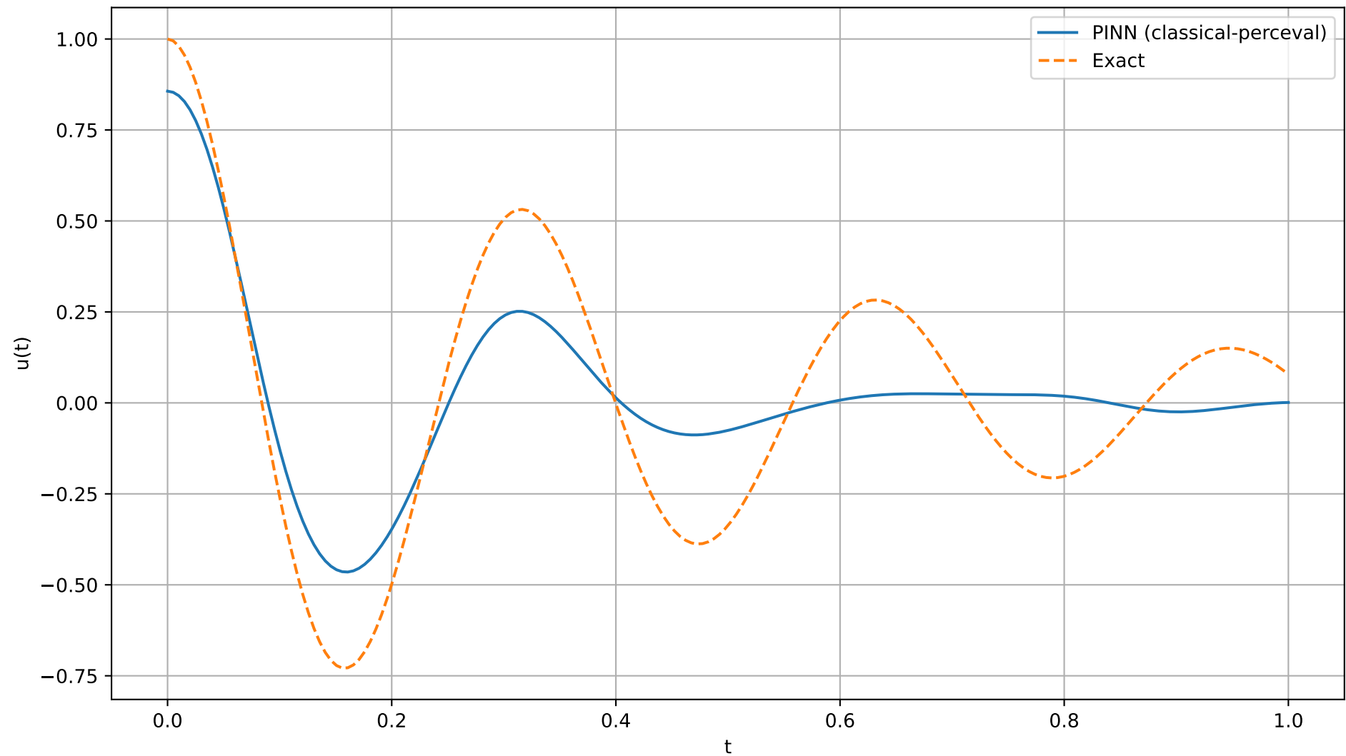
Final Prediction vs Exact
