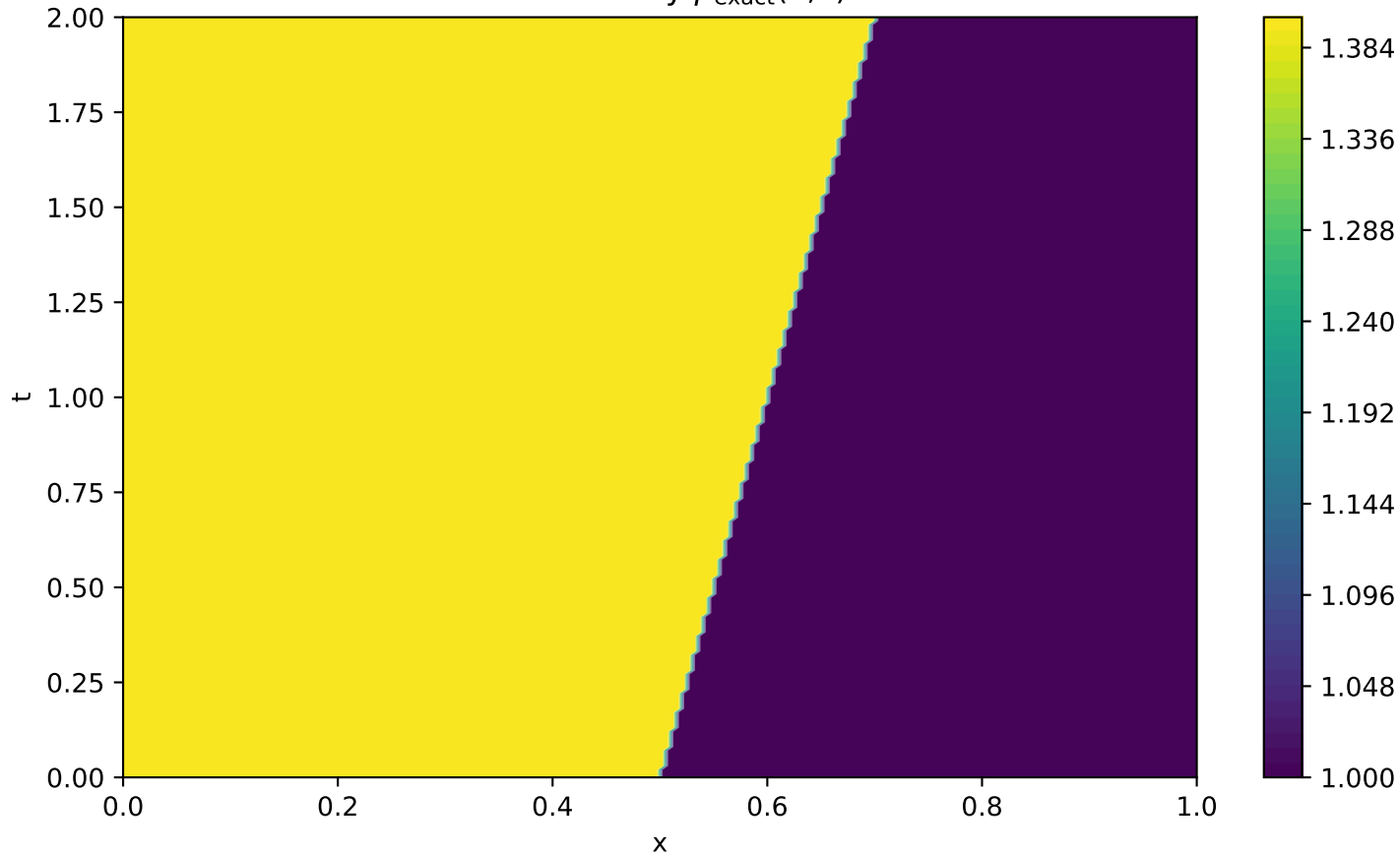
Exact density \rho_{\text{exact}}(x, t)
