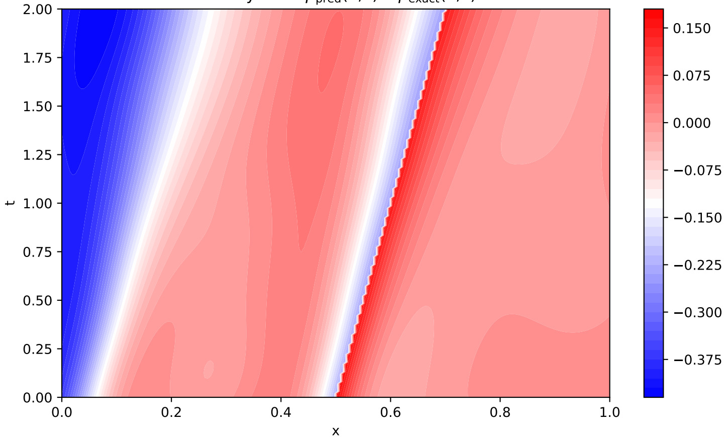
Density error \rho_{\text{pred}}(x, t) - \rho_{\text{exact}}(x, t)
