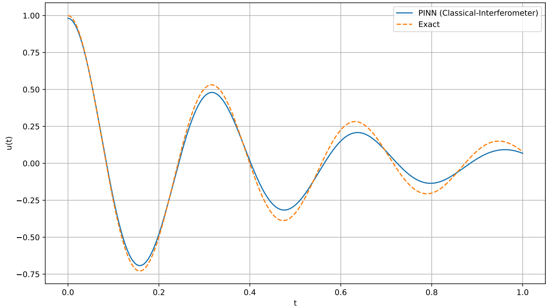
92.33s - 1800 epochs
