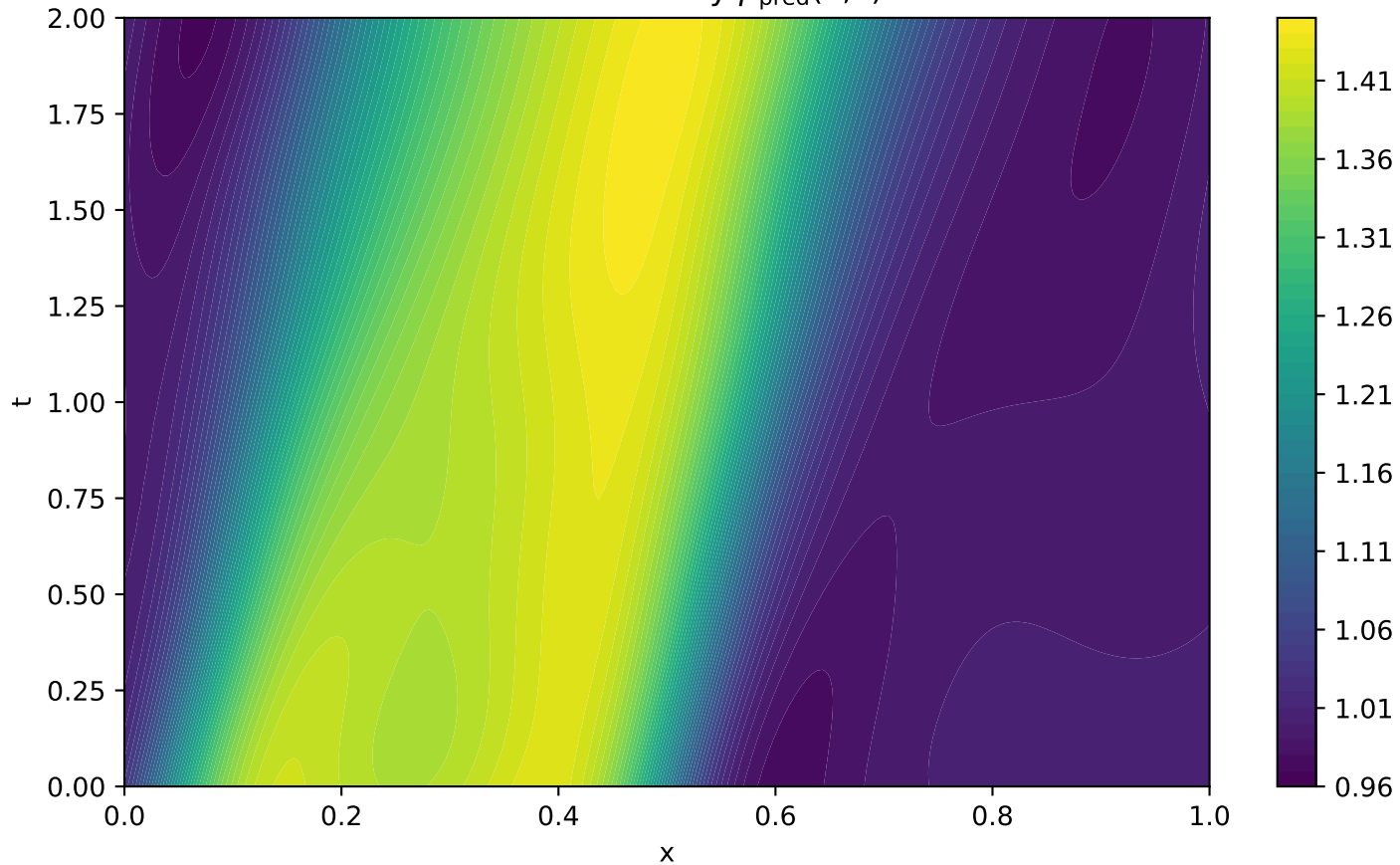
Predicted density \rho_{\text{pred}}(x, t)
