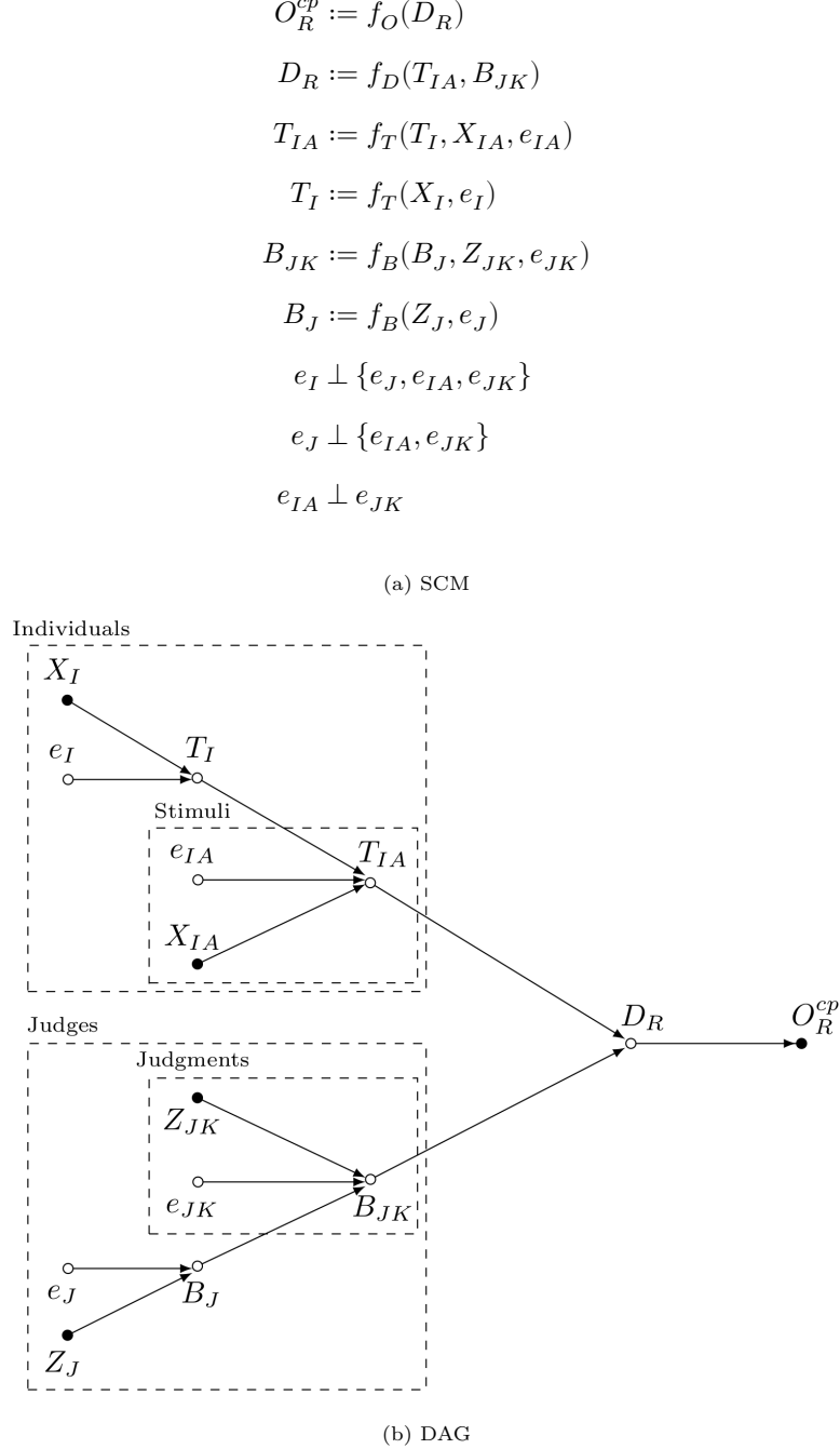
Figure 6: Conceptual-population model (CPM), final vectorized form.
