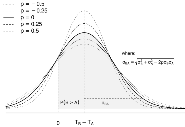
Figure 3: Discriminial Difference distribution under varying levels of correlation between stimuli
