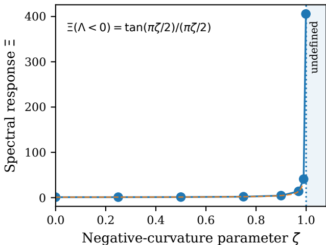
(c) Negative curvature approaches a caustic
